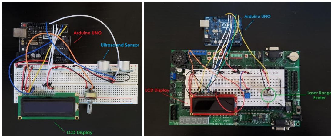
Figure 1: The Ultrasonic sensor and Laser Range Finder setups used to make measurements
