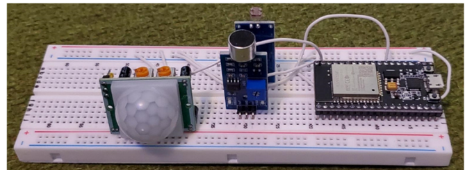
FIGURE II SENSOR BASED REAL-TIME ROOM OCCUPANCY TRACKER (By: Donovan Porter and Hunter Ylitalo)
