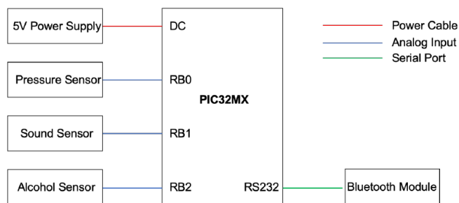
FIGURE I BLOCK DIAGRAM OF DRUNK-DRIVER TEST SYSTEM (By: Yizhi Fan and Mingdi Bian)
