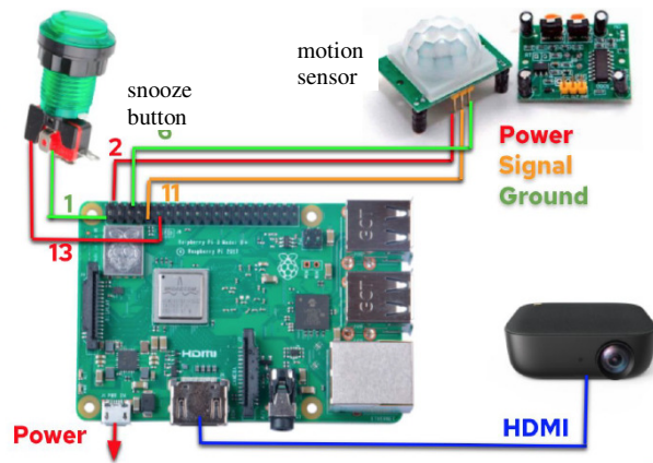
FIGURE III SMART ALARM SYSTEM
