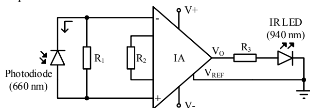
Fig. 3. Circuit for wavelength conversion from 660 nm to 940 nm.
