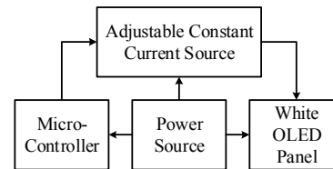
Fig. 1. Scheme of the OLED lamp used as an optical transmitter in the study.
