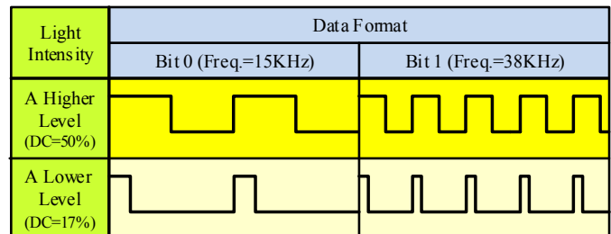
Fig. 2. Rules for carrier signals to implement data transmission and illumination at the same OLED panel.
