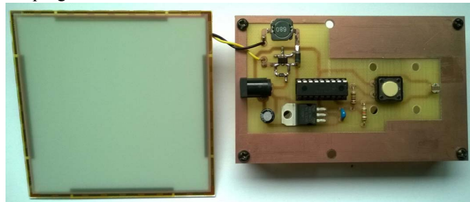
Fig. 4. A white OLED panel and its controller for a lamp prototype. Besides used for illumination, it is also operated as an optical transmitter.
