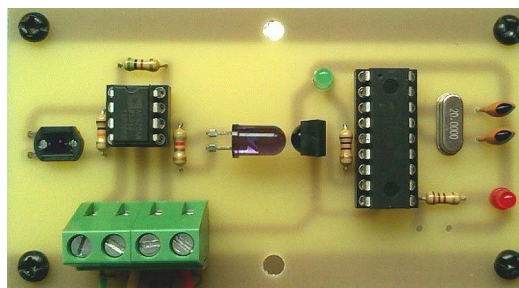
Fig. 5. An optical receiver works with the transmitter (Fig. 4). The conversion of the wavelength shown in Fig. 3 is implemented at the left half part.
