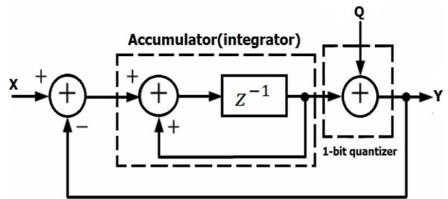
Fig 4. Block diagram of 1 st \Sigma\Delta modulator.
