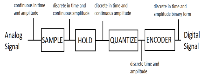
Fig 1: Nyquist rate ADCs.
