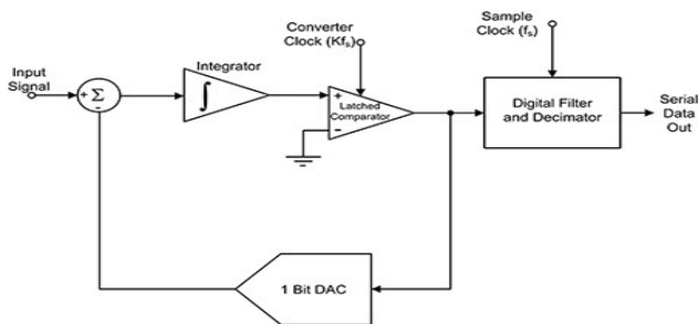
Fig3. Block diagram of A/D system \Sigma\Delta .
