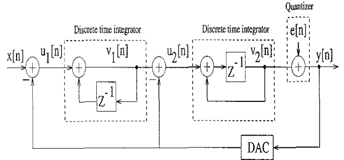
Fig. 6. Block diagram of 2 nd \Sigma\Delta modulator.
