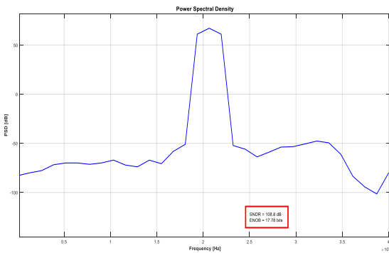
Fig 10. Frequency response of the power spectrum in the output of the 2 nd order \Sigma\Delta converter with the expected 18-bit accuracy.
