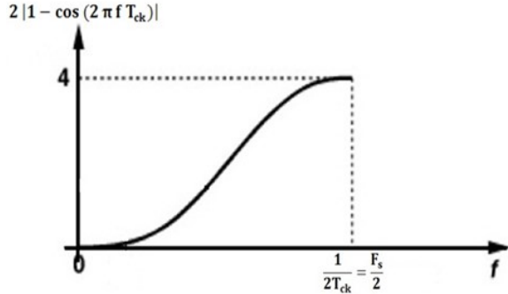
Fig. 5. Noise Shaping in the sigma-delta first order.
