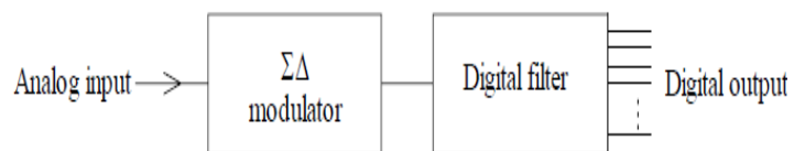
Fig 2: Oversampling ADCs.
