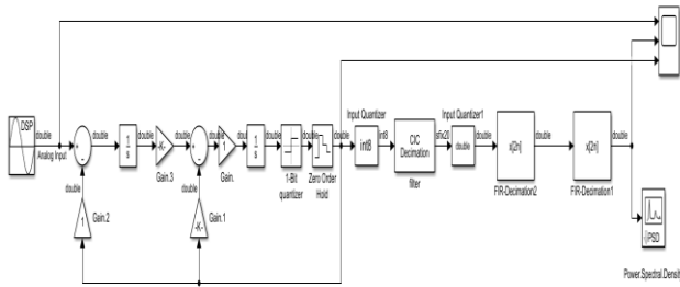
Fig7. The Sigma Delta A/D model.
