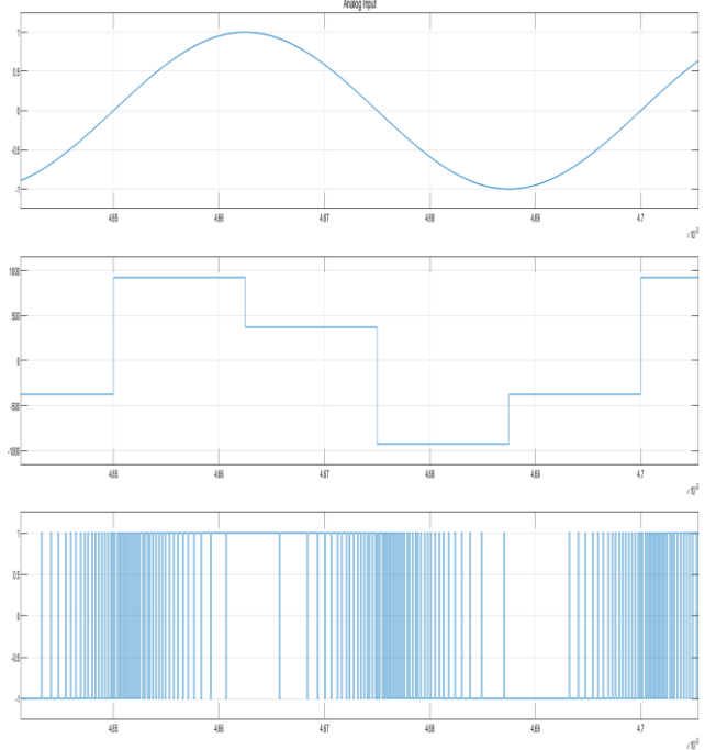
Fig 8. Second order modulator transient response for a sine-wave input of 20 KHz.
