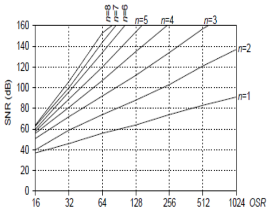
Figure 11: Relation between S/N and OSR.
