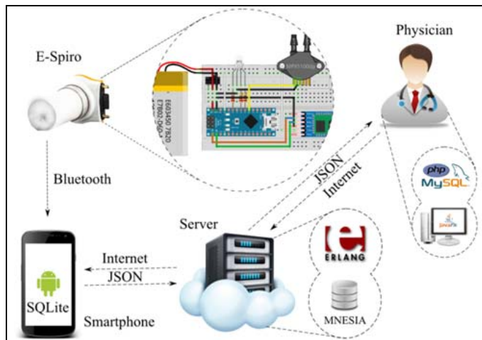
Figure 1. General system design
