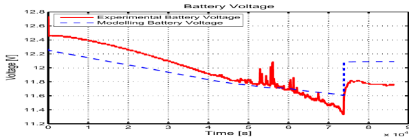
Fig. 4. Battery Voltage from the First Case Study
