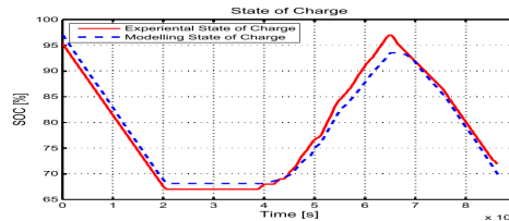
Fig. 8. State of Charge in the Second Case Study
