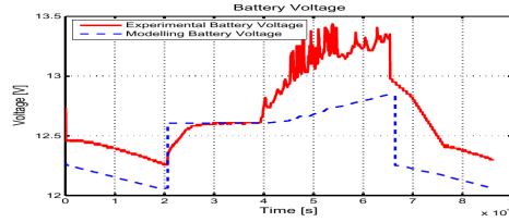
Fig. 7. Voltage of the Battery in the Second Case Study
