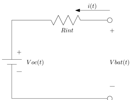
Fig. 1. Circuitual Diagram of the Theoretical Model
