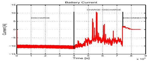
Fig. 3. Current Charge-Discharge of the First Case Study
