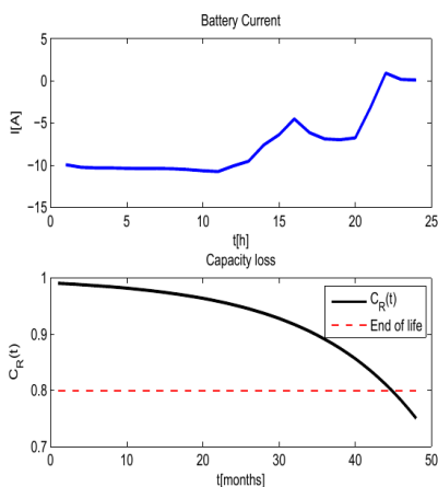
Fig. 9. Loss of Capacity for the First Case Study
