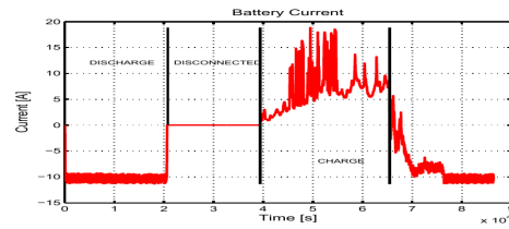
Fig. 6. Current of Charge-Discharge in the Second Case Study
