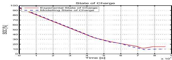
Fig. 5. State of Charge in the First Case Study
