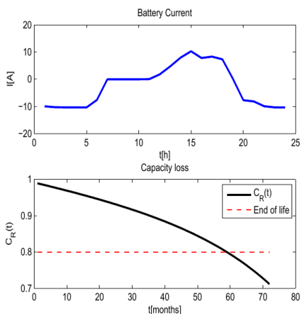
Fig. 10. Loss of Capacity for the Second Case Study
