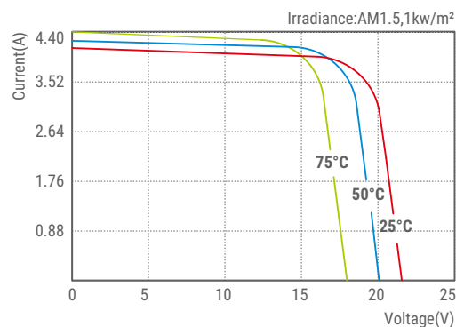
SLP060-12U I-V Curves
