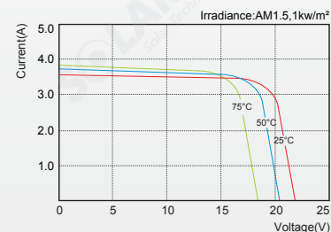
SLP060-12C1D2 I-V Curves
