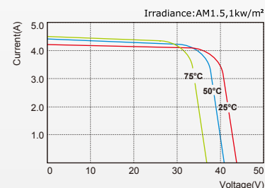
SLP140-24 I-V Curves
