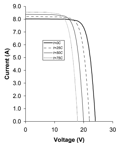
BP 3130 I-V Curves
