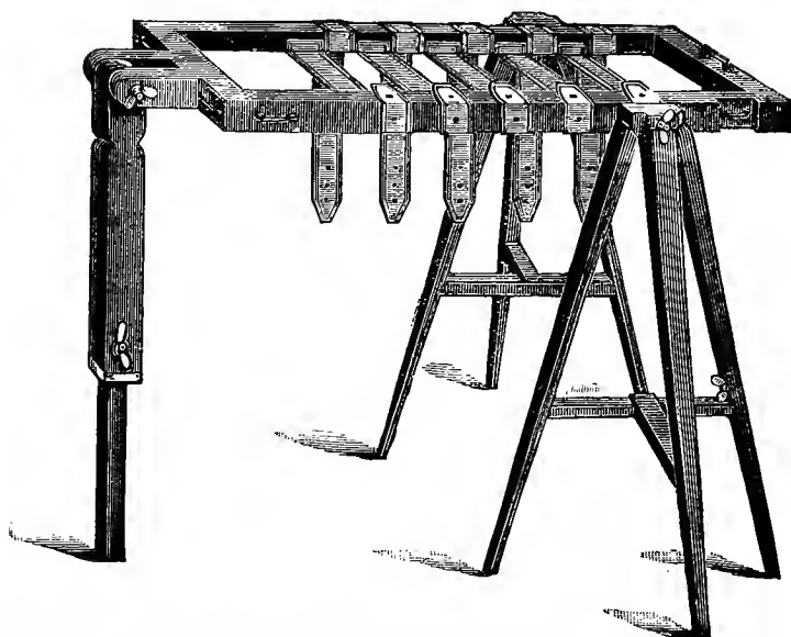
FIG. 146.—Hill's animal table. The table can be raised or lowered at one end, or be reversed.
