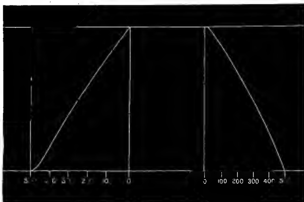
FIG. 56.—Elasticity curve of rubber tubing. The figures represent weights in grms. (M.S.P.)
