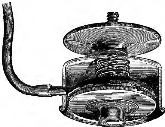
FIG. 117.—Marsy's cardiograph. The tube is connected with a recording tambour. Pressure is adjusted by the screw and spring.
