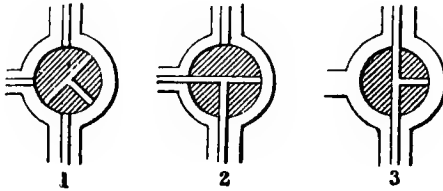
FIG. 185.—The three-way tap of the mercury pump.
