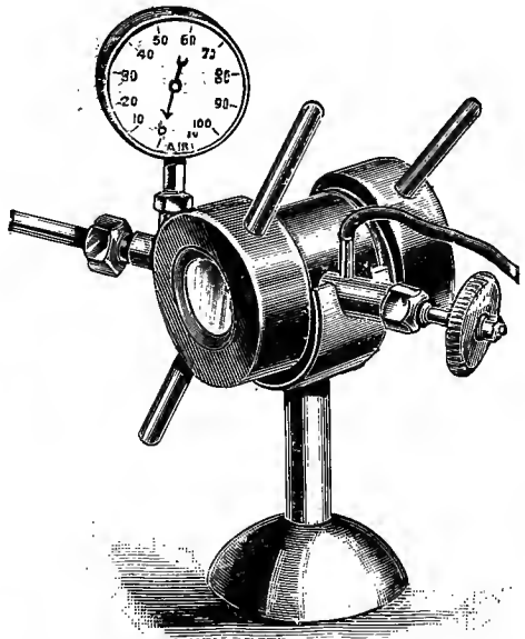
FIG. 190.—Hill's apparatus for studying effects of increased atmospheric pressure. Thick glass discs, provided with leather washers, close the ends of the chamber.
