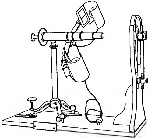
FIG. 210. —The ophthalmometer.
