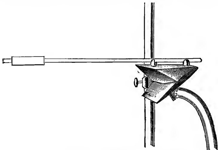
FIG. 208.—Brodie's bellows recorder. The bellows are made of aluminium plates and peritoneal membrane.
