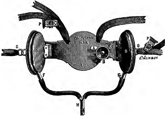
FIG. 177.—A stethograph employed to record the respiration and cardiac impulse of the rabbit or cat. The tamboours press on either side of the thorax. The T tube leads to a recording tambour.
