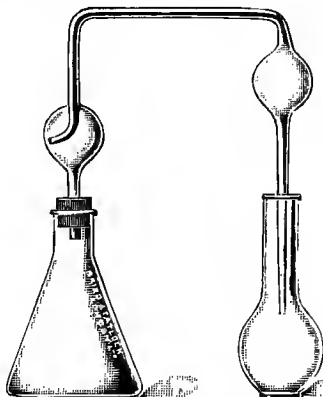
FIG. 239.—Apparatus for determination of total nitrogen.
