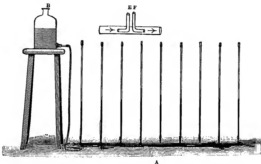
FIG. 170.—Schema to show the velocity and resistance heads. B, Pressure bottle. A, Tube with picnimeters. E F, Pitot tubes.
