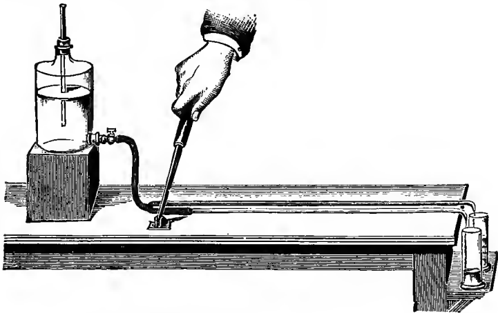
FIG. 132.—Schema to show the flow in rigid and elastic tubes. (Marey.)
