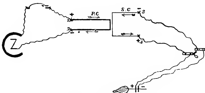
FIG. 16.—Diagram of an induction-coil and its connections.
