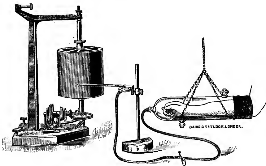
FIG. 175.—Limb plethysmograph.
