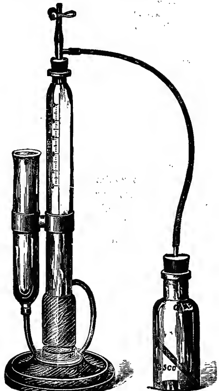
FIG. 243.—Gerrard's urea apparatus.
