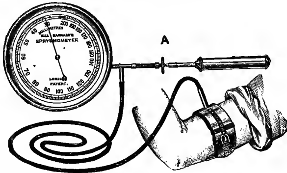
FIG. 128.—Spring sphygmometer. The leather armlet encloses a rubber bag. The bicycle pump is used to raise the pressure. The spring manometer indicates the maximal pulsation and the pressure.
