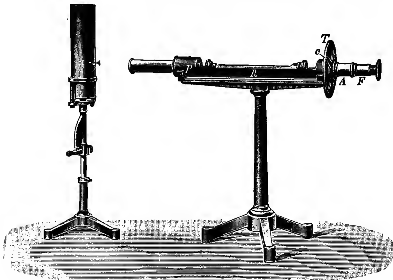
FIG. 222.—Polarimeter of Mischerlich with Laurent's polariser. P , polariser and device for obtaining half shadow; R , fluid container; T , scale with vernier c attached to pointer; A , compensator and analyser; F , lens.
