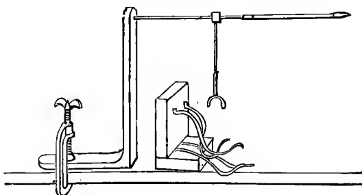
FIG. 66.—Spring ergograph. (Porter.)
