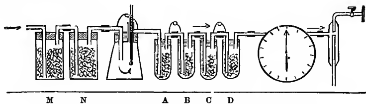
FIG. 183.—The Haldane-Pembrey respiration apparatus for the mouse.
