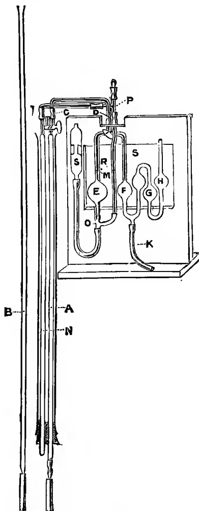
FIG. 179.—Haldane's gas analysis apparatus.
