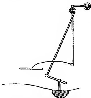
FIG. 123.—Arrangement of levers in Dudgeon's sphygmograph.
