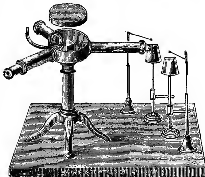
FIG. 230.—Compound spectroscop.
