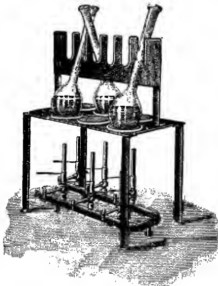
FIG. 238.—Apparatus for determination of total nitrogen.
