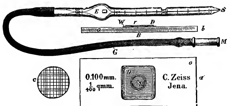
FIG. 130.—The Thoma-Zeiss haemocytometer.
