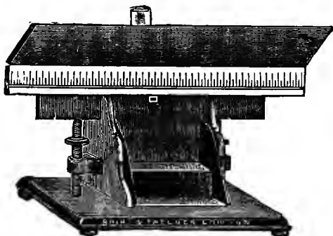
FIG. 87.—Scale and lamp for the reflecting galvanometer.
