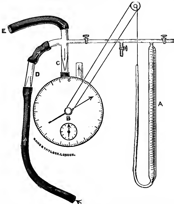
FIG. 182. Zuntz respiration apparatus. The subject expires through the meter. The inlet and outlet tubes are controlled by valves D and C, made of pieces of intestine which have been soaked in glycerine. A small sample of the expired air is steadily drawn off into the burette A by the escape of mercury from the tube which is lowered by the revolution of the meter B. The meter gives the total volume of air breathed. The measured sample in the burette is analysed by Haldane's gas apparatus.
