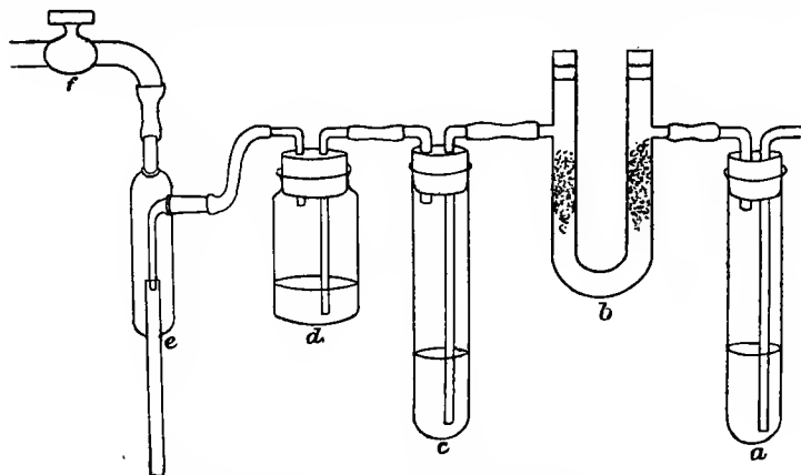
FIG. 247.—Folin's apparatus for estimating ammonia.
