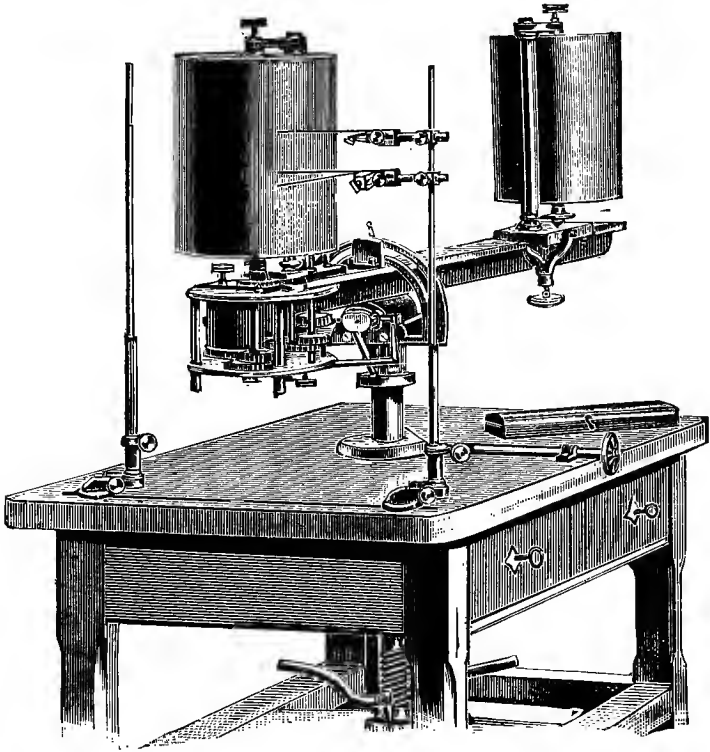
FIG. 140.—The kymograph.
