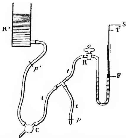
FIG. 137.—Arrangement of cannula, pressure bottle, and mercurial manometer for recording blood pressure. C, cannula; p, p', clips; F, float; S, writing style.
