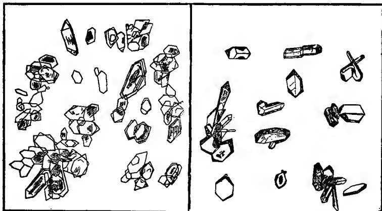
FIG. 240.—Urea nitrate.
