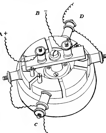
FIG. 8B.—Universal key (Gotch). The key is used by rotating the arm containing the screws connected with the wires A and B , which come from the battery. In the position shown the current flows from the wire of C to that of D ; if rotated through 45^\circ there is a complete double break of the battery-circuit; if rotated through 90^\circ then the current is remade and the current flows from the wire of D to that of C .
