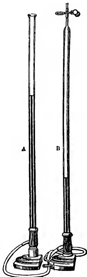
FIG. 180.—Hempel's burette for collecting a sample of expired air.
