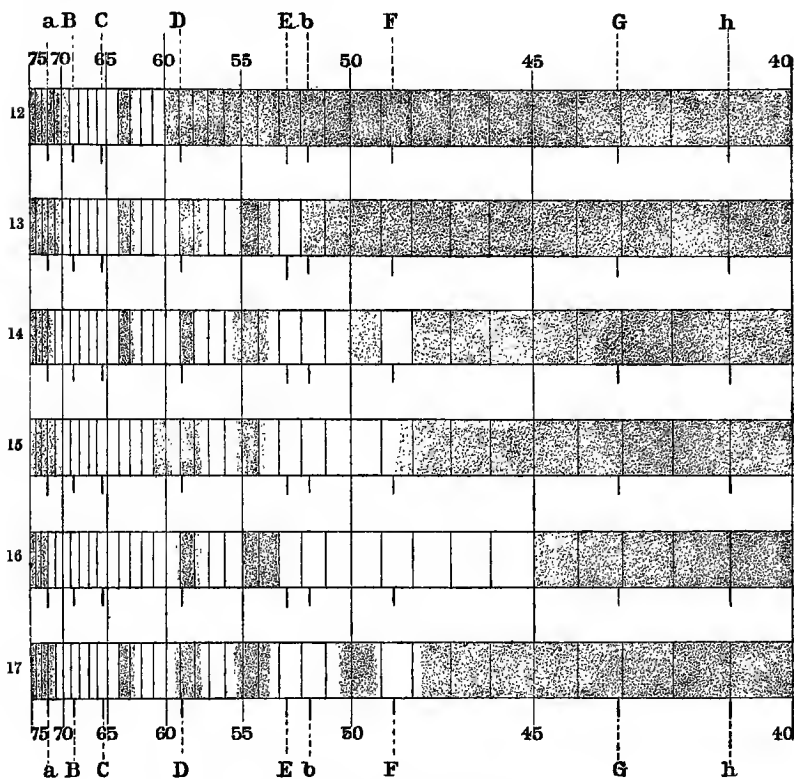
FIG. 232.—Absorption-spectra.
