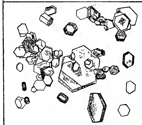
FIG. 250.—Cystine. \times 350 .
