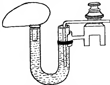
FIG. 74.—Unpolarisable electrode. Burdon-Sanderson's pattern.
