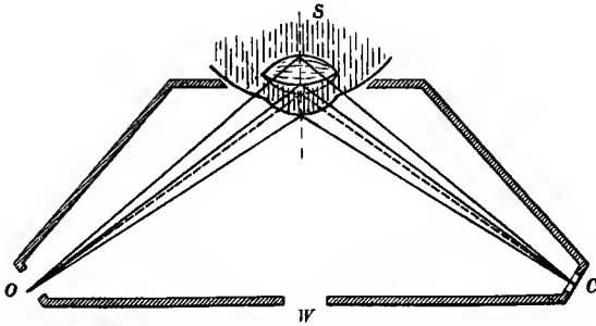
FIG. 214.—Diagram of the course of the rays of light in the phakoscope.
