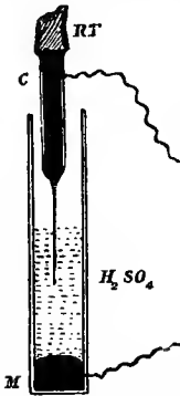
FIG. 88.—Diagram of the capillary electrometer.
