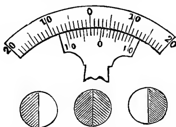
FIG. 223.—Diagram of scale and field of vision of polarimeter. Above is represented the scale for measuring the compensation necessary. In the position represented in the diagram the reading is 2.7 dextro rotation. The lower part of the diagram shows the three appearances of the field of the polarimeter, the central one representing the appearance at zero, i.e. when there is no rotation.
