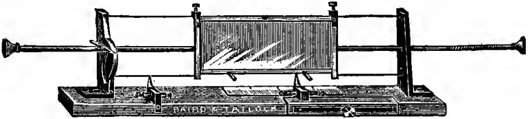
FIG. 63. —The spring myograph.
