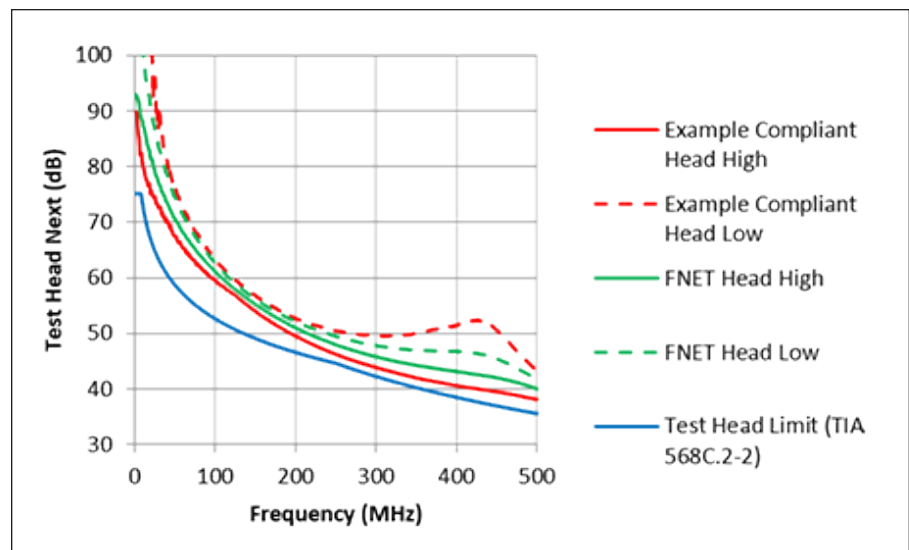
Figure 3: Variation compliant test heads
