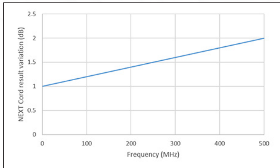
Figure 5: Maximum cord result variation
