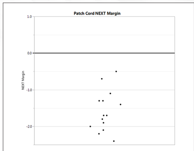
Figure 8: Patch cords from channels in figure 6 measured by CommScope
