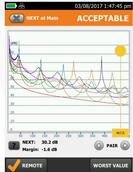
NEXT plot data
