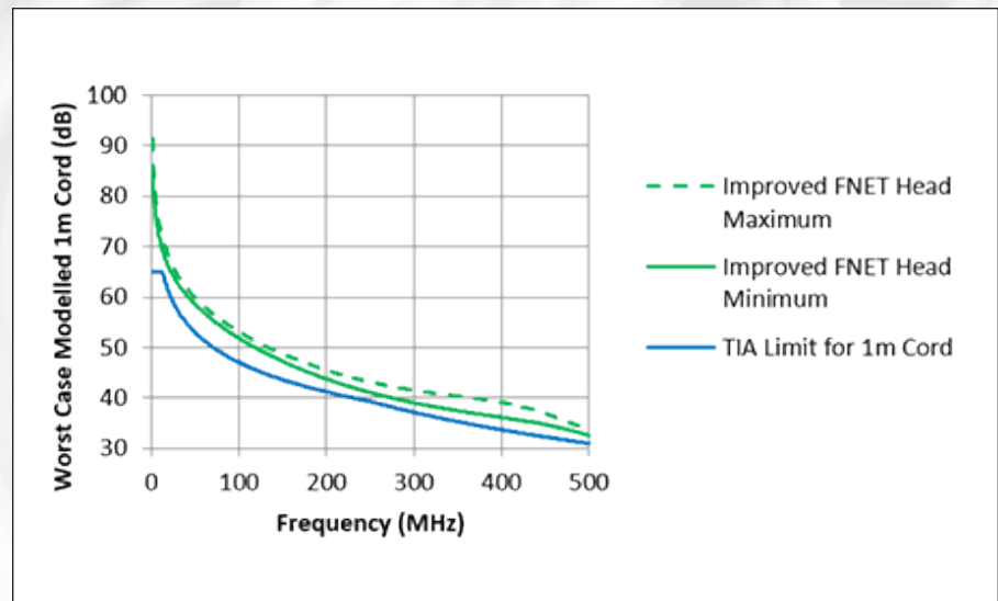
Figure 4: Study of variation seen on 1 m cord results
