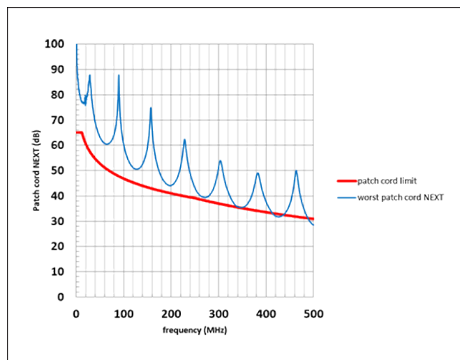
Figure 9: Worst case patch cord NEXT frequency response measured by CommScope
