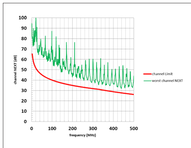
Figure 10: Worst case channel NEXT frequency response measured by CommScope
