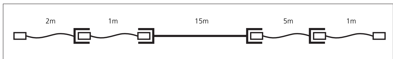
Figure 6: This is one of the reference modeling implementation in ANSI/TIA-568.C-2 Annex J
