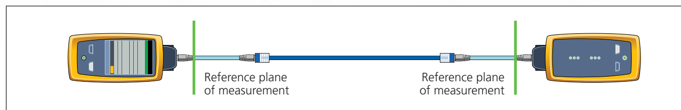
Figure 1: Channel reference planes
