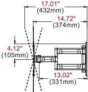
SIDE VIEW EXTENDED +/- 15° TILT
