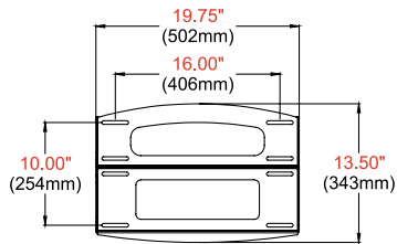
WALL PLATE
