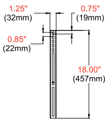
ADAPTOR BRACKET
