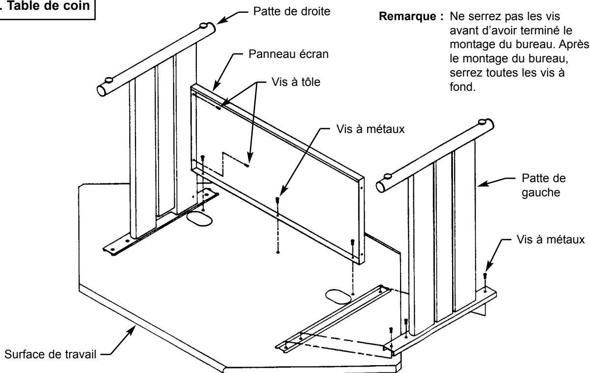
Figure 2. Table de coin
