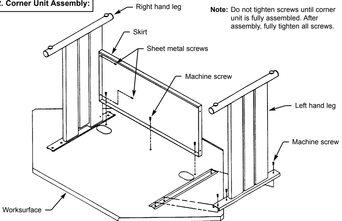
Illustration 2. Corner Unit Assembly:
