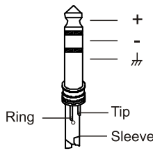
TRS Type Balanced
