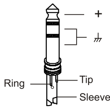
TRS Type Unbalanced
