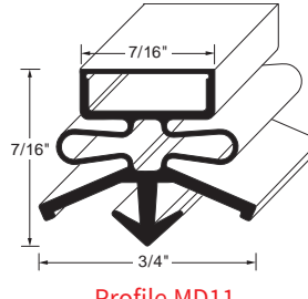
Profile MD11 Order No. 90-1028 (Black) or 90-1043 (Gray)
