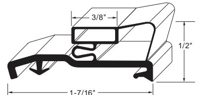
Profile MD15 Order No. 90-1029
