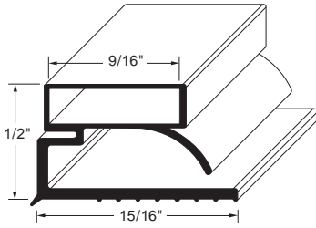
Profile MS5 Order No. 90-1003
