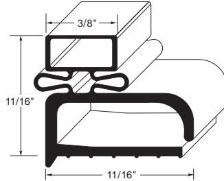
Profile MS2 Order No. 90-1001
