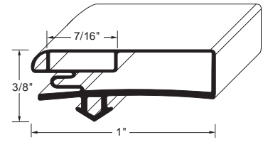
Profile MD7 Order No. 90-1025
