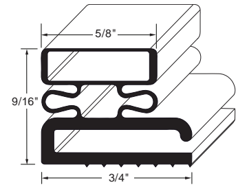
Profile MS3 Order No. 90-1041 (Black) or 90-1002 (Gray)
