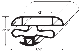
Profile MD8 Order No. 90-1026
