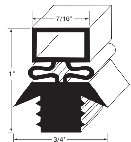
Profile MP4 Order No. 90-1034
