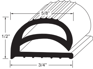
Profile CS1 Order No. 90-1000
