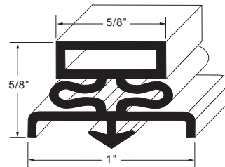
Profile MD6 Order No. 90-1005
