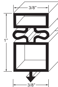
Profile MD26 Order No. 90-1030
