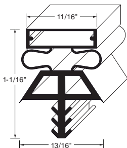
Profile MD30 Order No. 90-1032
