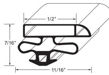
Profile MD41 Order No. 90-1040
