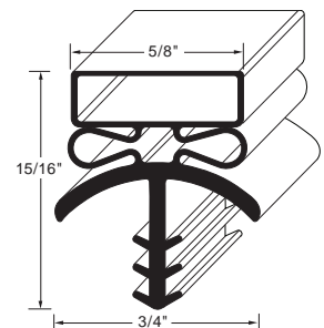
Profile MD28 Order No. 90-1031
