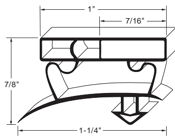
Profile MD39 Order No. 90-1033
