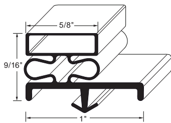
Profile MD23 Order No. 90-1042 (Black), 90-1004 (Gray PVC) or 90-1044 (Gray Santoprene™)
