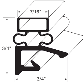
Profile MS8 Order No. 90-1035
