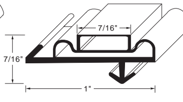
Profile MD9 Order No. 90-1027
