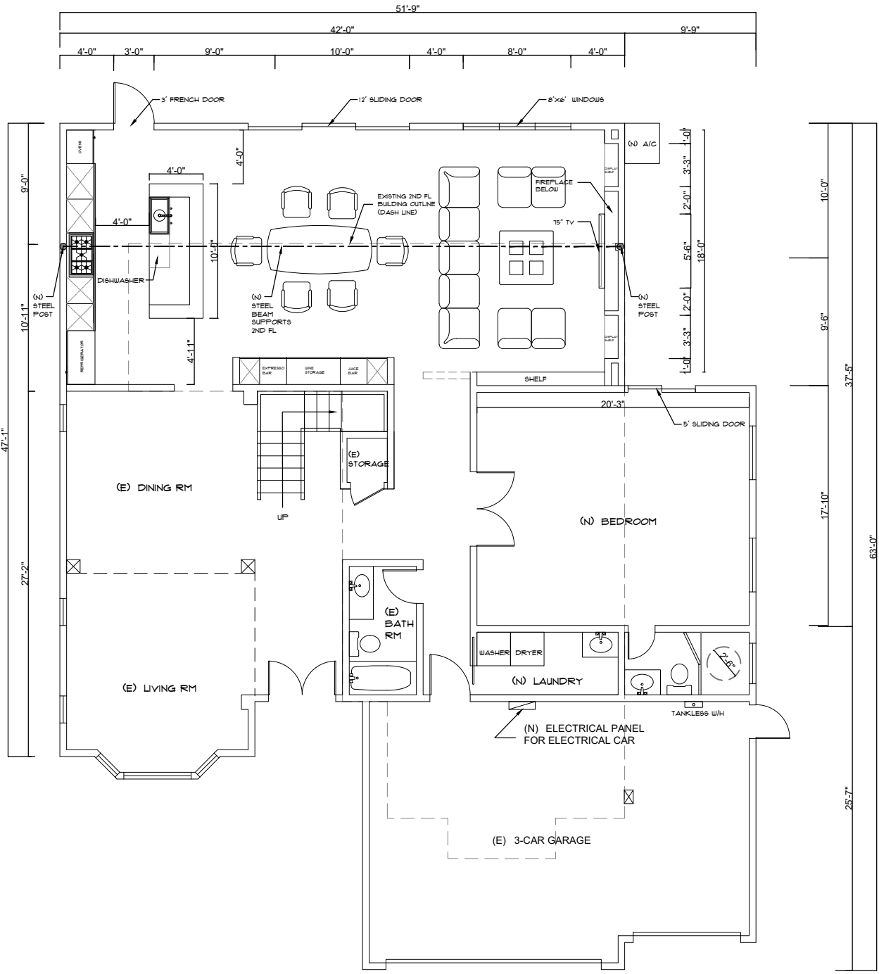
FLOOR PLAN DESIGN OPTION ON 06/08/2018 N.T.S
