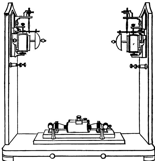
Fig. 93.—Bright's Acoustic Telegraph.
