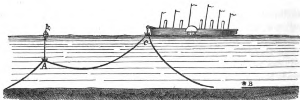
Fig. 91.—Diagram showing final arrangement for picking up cable of 1865.
