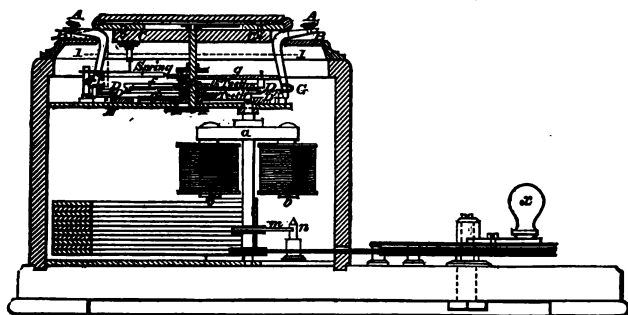
Fig. 111.—Professor Wheatstone's Alphabetical Telegraph—Sending Apparatus (Section).
