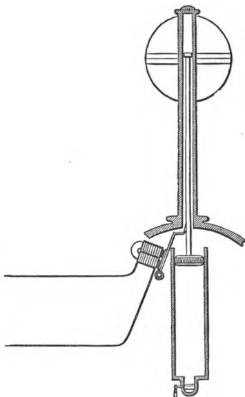
Fig. 127.—Time-ball Apparatus. Section.
