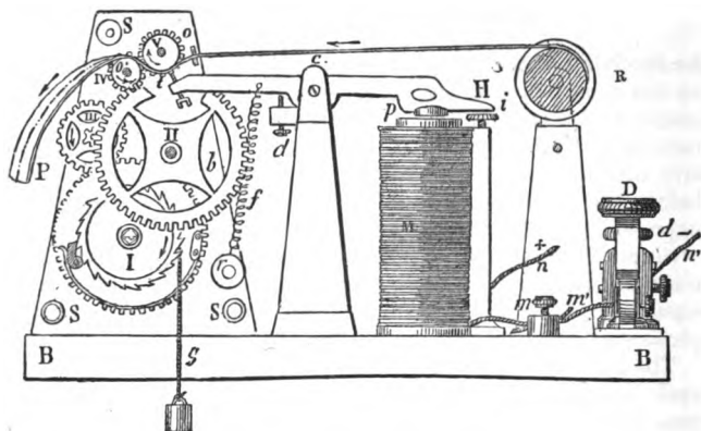
Fig. 102.—Morse's American Recording Telegraph.
