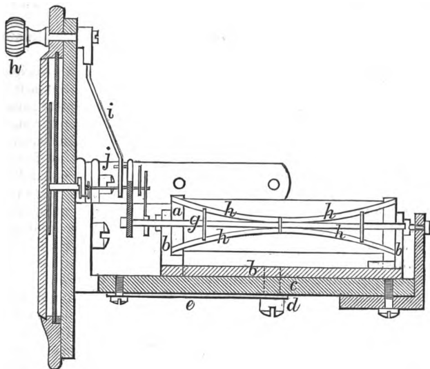
Fig. 112.—Professor Wheatstone's Alphabetical Instrument—Indicating Apparatus (Section).
