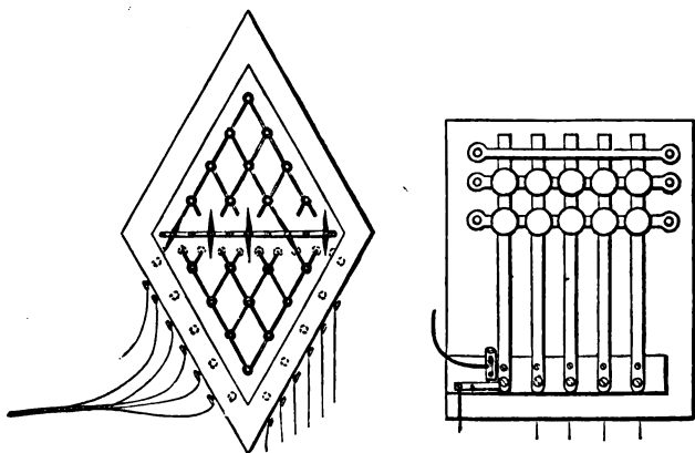
Fig. 16.—Cooke and Wheatstone's five-needle Telegraph, 1837.
