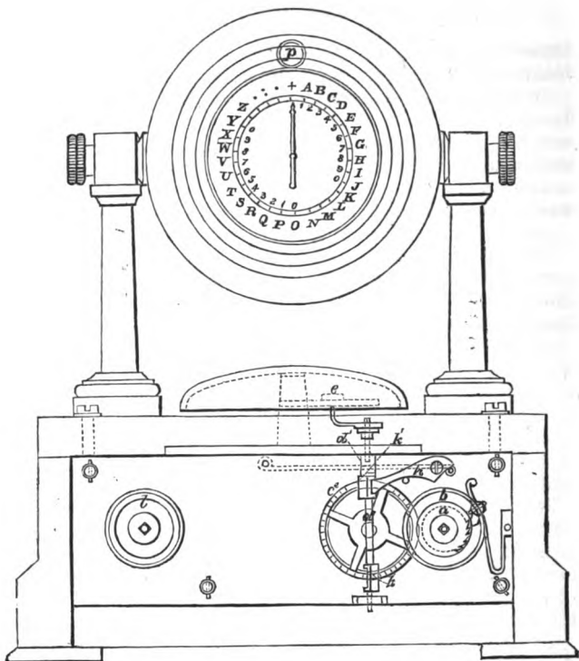
Fig. 109.—Professor Wheatstone's Alphabetical Instrument. (Receiving Apparatus and Alarm.)
