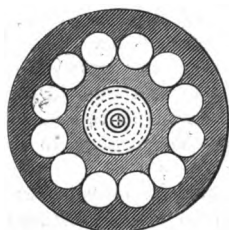
Fig. 75.—Side view and section of the Persian Gulf cable; actual size.
