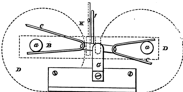
Fig. 133.—Walker's Semaphore Railway Telegraph. Diagram of indicating apparatus.
