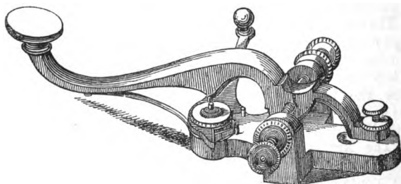
Fig. 105.—Morse Commutator Key.
