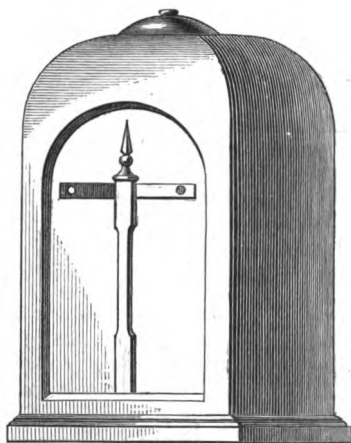
Fig. 132.—Electro-magnetic Telegraph Semaphore. Invented by Messrs. Walker.
