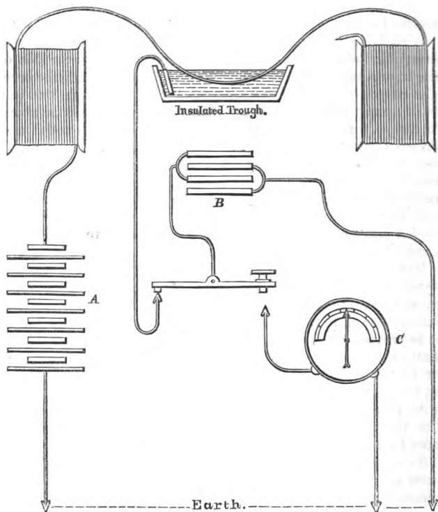
Fig. 74.—Joint testing by accumulation.
