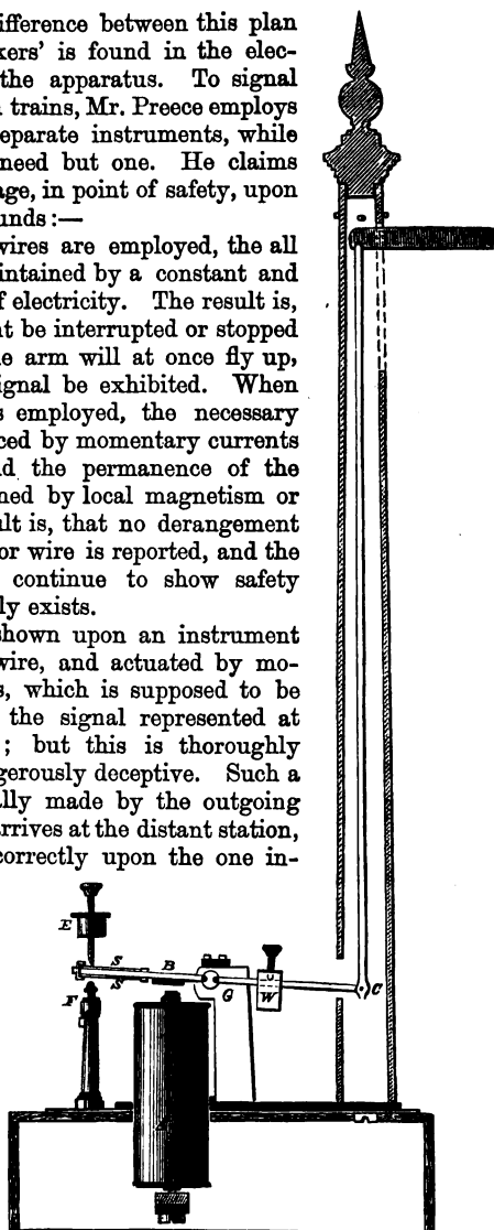
Fig. 135.—Preece's Semaphore Telegraph. (Section.)
