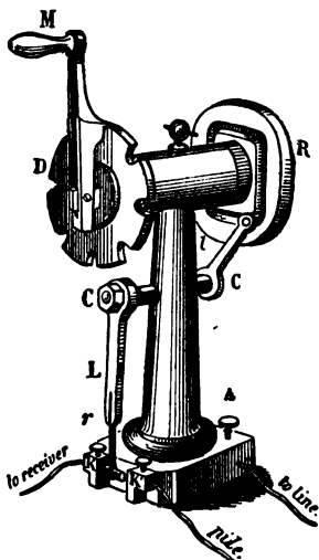
Fig. 101.—Sending Apparatus.
