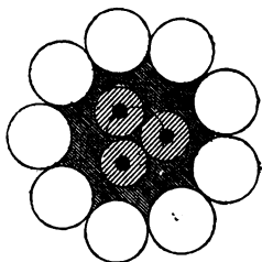
Fig. 66.—Great Belt.
