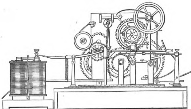
[Fig. 125.—Hughes' American Printing Telegraph.]
