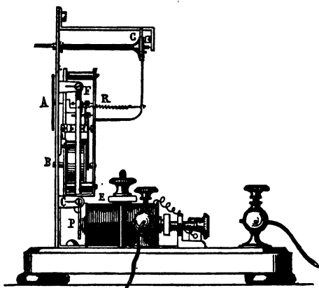
Fig. 115.—Breguet's Alphabetical Instrument (Section).
