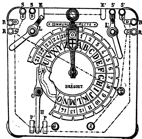
Fig. 114.—Breguet's Sending Apparatus.
