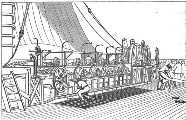
Fig. 88.—Paying-out machine, 1865—6.
