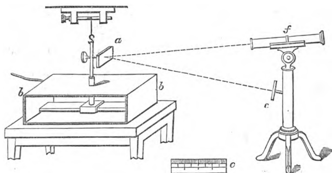
Fig. 17.—Gauss and Weber's Telegraph.
