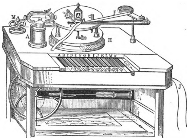
Fig. 123.—House's American Printing Telegraph.
