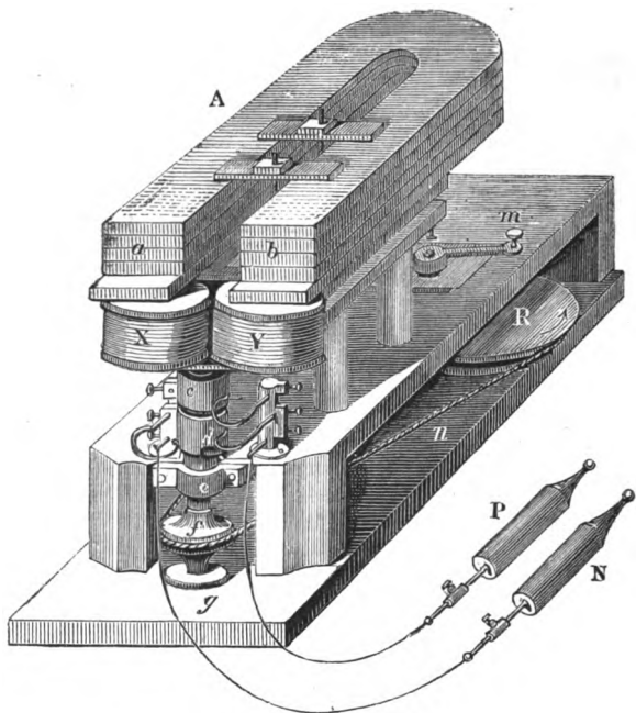
Fig. 4.—MAGNETO-ELECTRIC MACHINE.
