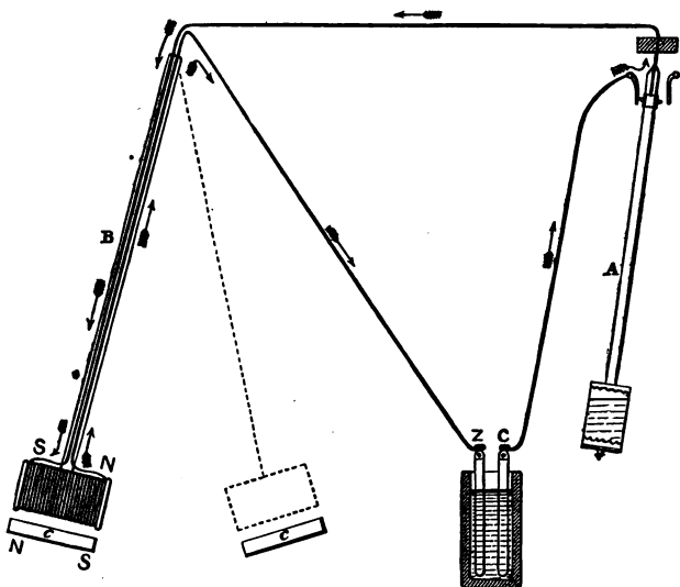
Fig. 128.—Diagram exemplifying Jones' method of clock regulation by electricity.
