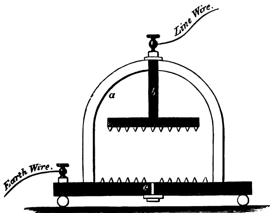
Fig. 46b.—Bright's rarefied air lightning protector.
