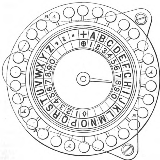
Fig. 110.—Professor Wheatstone's Alphabetical Telegraph—Sending Apparatus.
