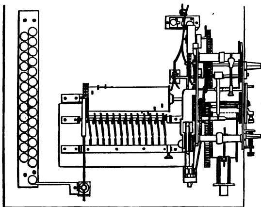
Fig. 126.—Hughes' Printing Instrument (Vertical Plan).
