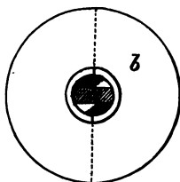
Fig. 86.—Atlantic galvanometer coil, mirror, and magnetic needle.
