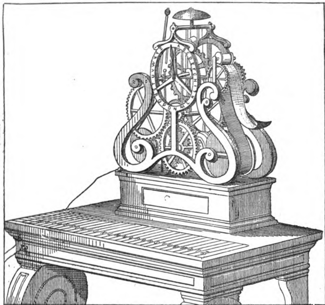
Fig. 124.—House and Brett's English type printer.
