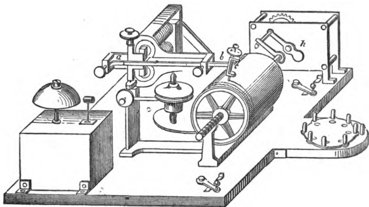
Fig. 106.—Froment's Recording Instrument.
