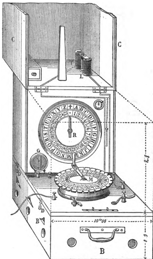
Fig. 116.—Breguet's Portable Alphabetical Instrument.
