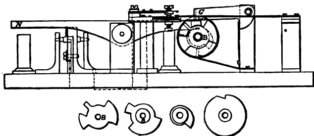
Fig. 92.—Transmitting Apparatus proposed for the Atlantic Cable.
