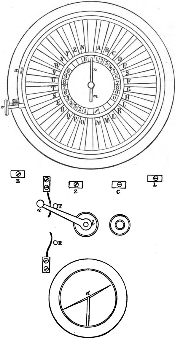
Fig. 117.—Siemens' Sending Keys and Indicator.
