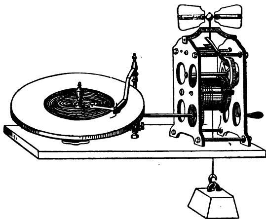
Fig. 107.—Bain's Electro-chemical Telegraph.
