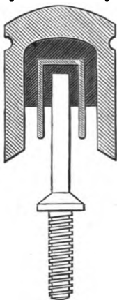
Fig. 36.—Double cup insulator.
