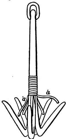
a, a, Springs to prevent the cable surging from the grapnel-flukes when hooked.
