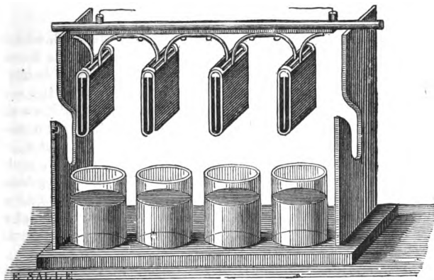
Fig. 20.—Wollaston's Battery.
