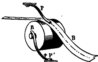
Fig. 108.—Bain's Electro-chemical Telegraph.
