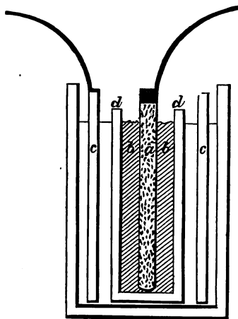
Fig. 25.—Marie Davy Battery.
