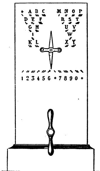
Fig. 94.—Single needle telegraph. Cooke and Wheatstone.
