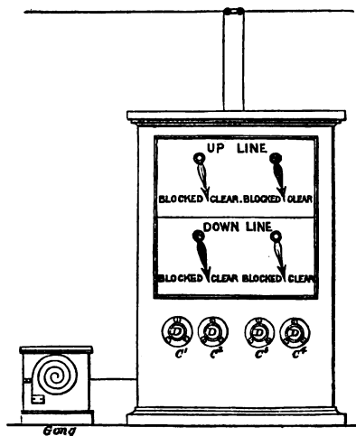
Fig. 136.—Tyer's Railway Telegraph .
