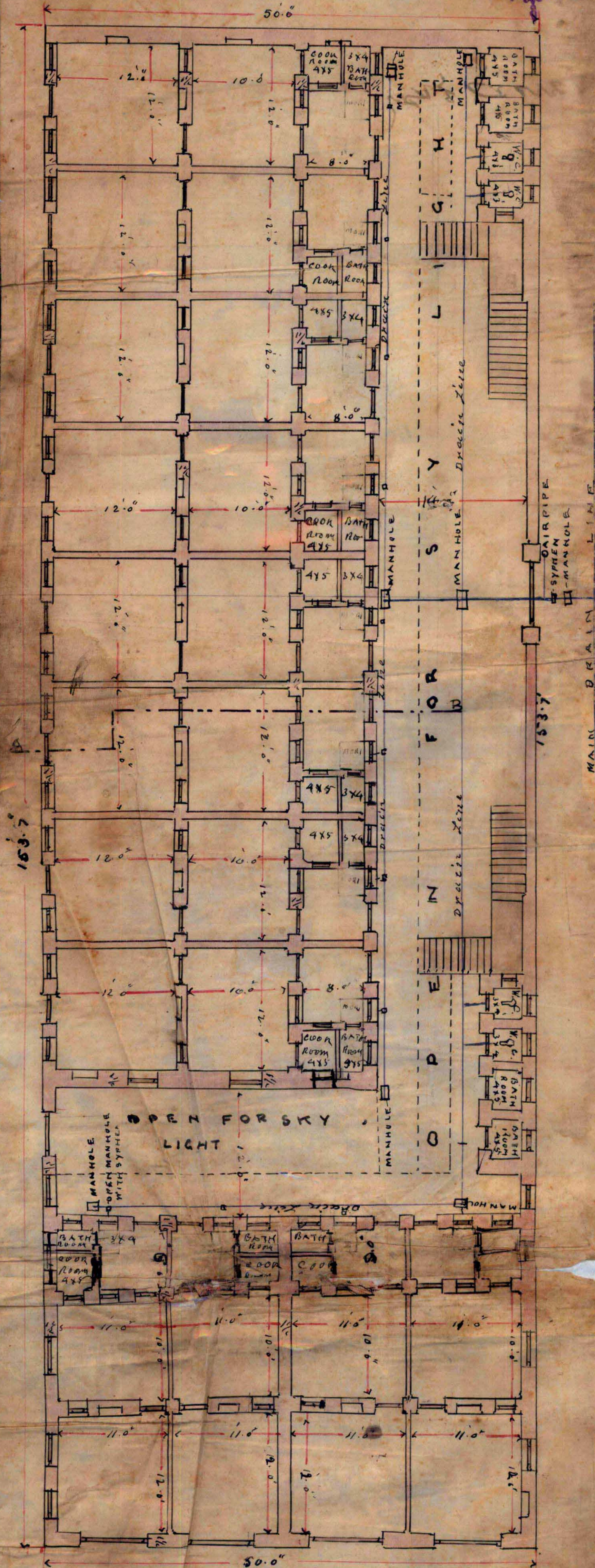
GROUND PLAN
