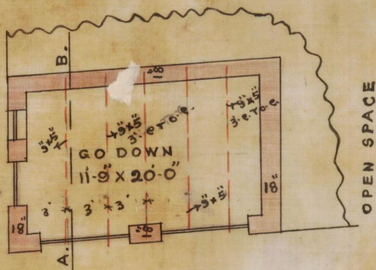
GROUND PLAN
