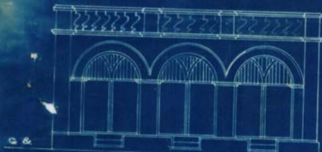
EAST ELEVATION
