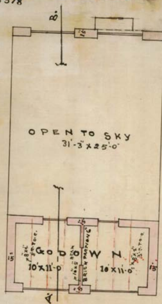
GROUND PLAN
