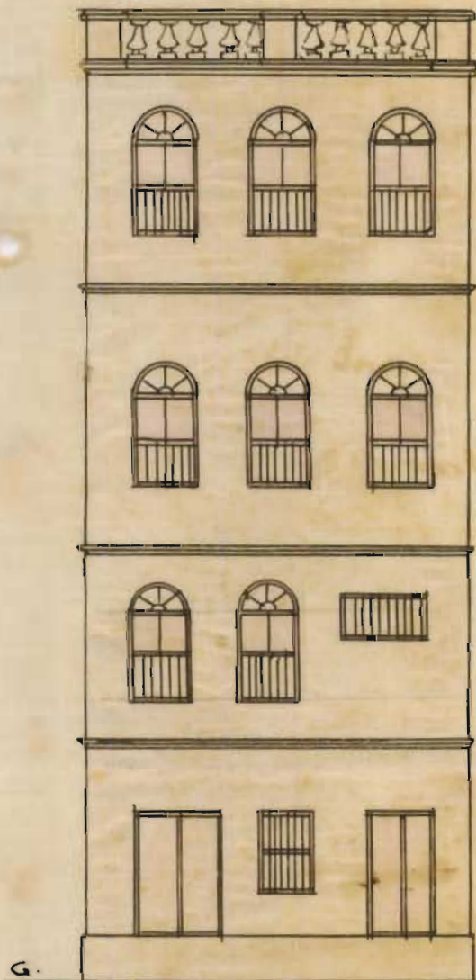
FRONT ELEVATION
