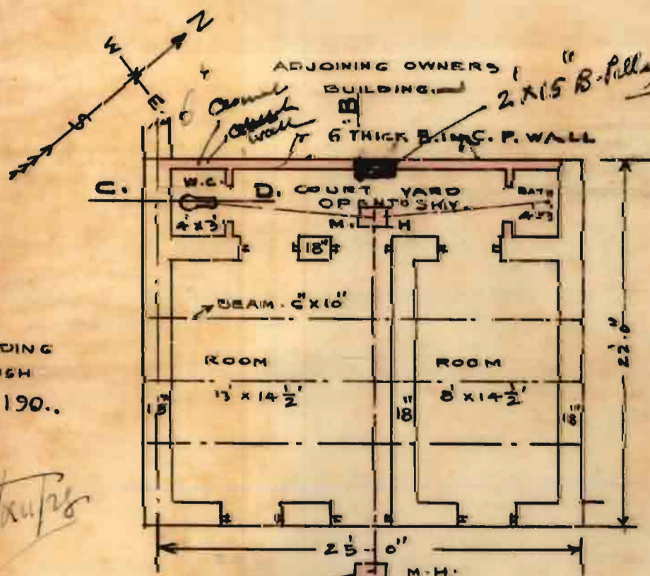
— GROUND PLAN —
