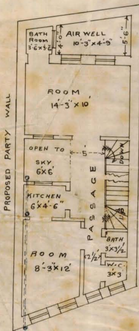
PLAN OF 1ST & 2ND FLOOR
