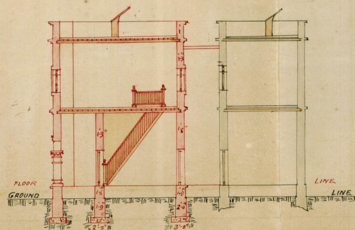
SECTION ON LINE A-B.
