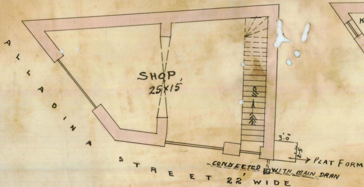
GROUND PLAN
