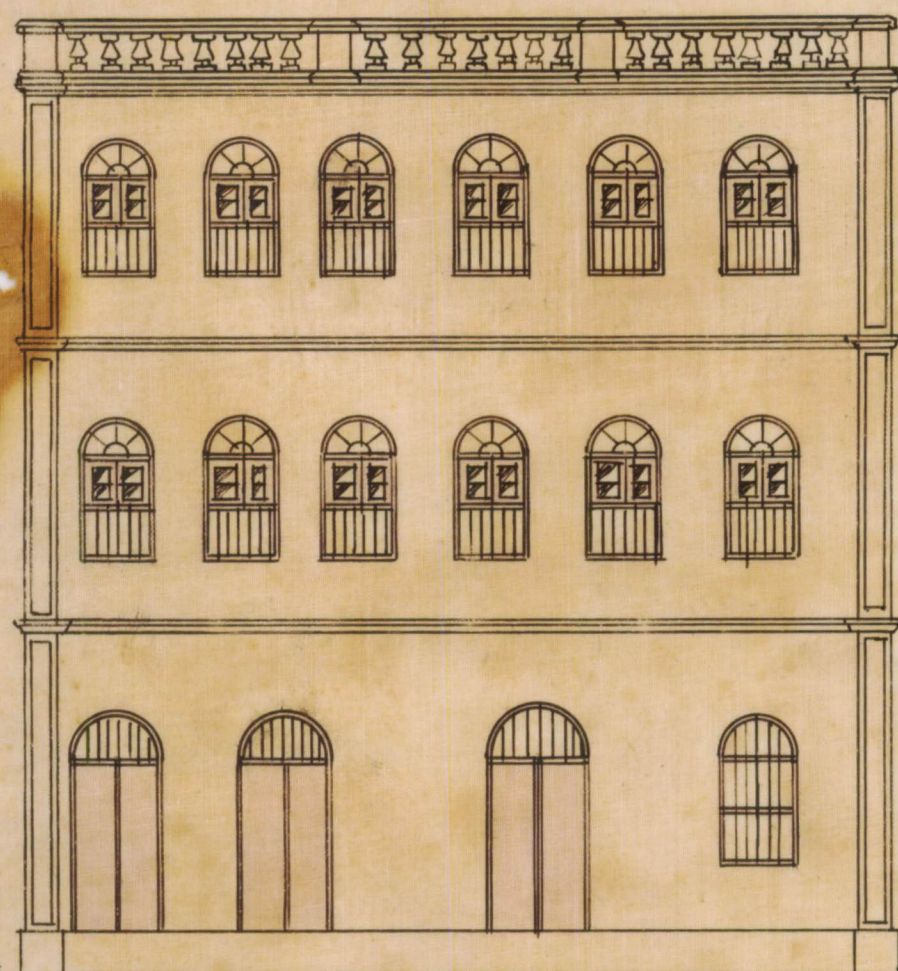
SOUTH ELEVATION
