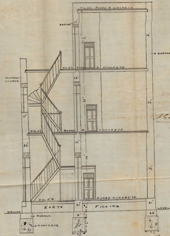
SHOWING PROPOSED BUILDING ON PLOT No 58, SHEET C.2. MUCHEE MEANEE QUARTER. SCALE 4" = 1"
