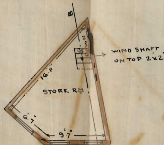
PLAN OF 1 ST FLOOR.
