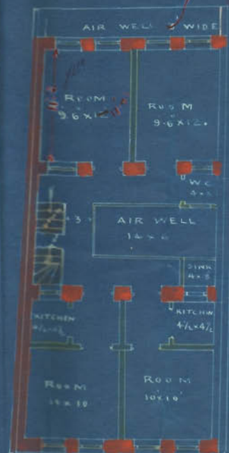
PLAN OF I & II FLOORS
