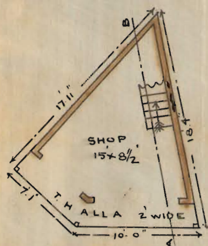
PLAN OF GROUND FLOOR
