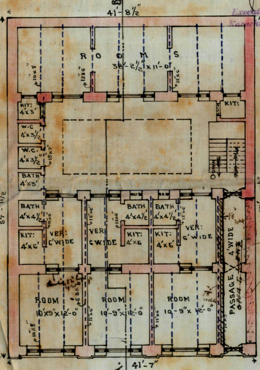
GROUND PLAN
