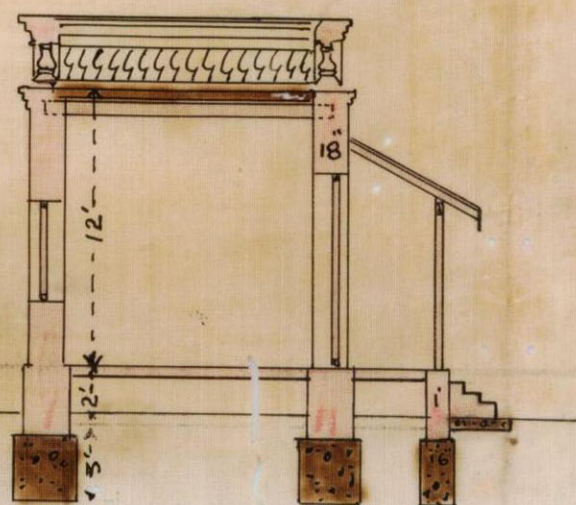
CROSS SECTION OF CHOWKIDAR'S QRS
