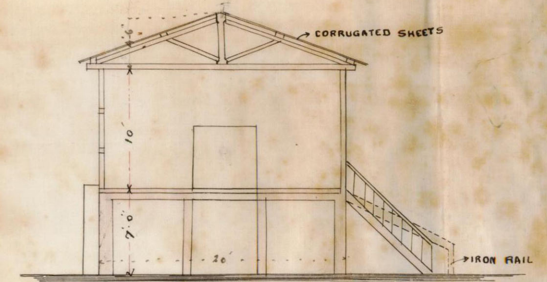
CROSS SECTION A.B.
