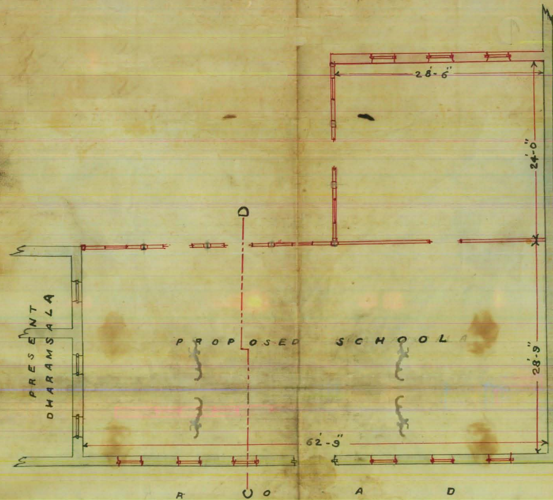
GROUND PLAN
