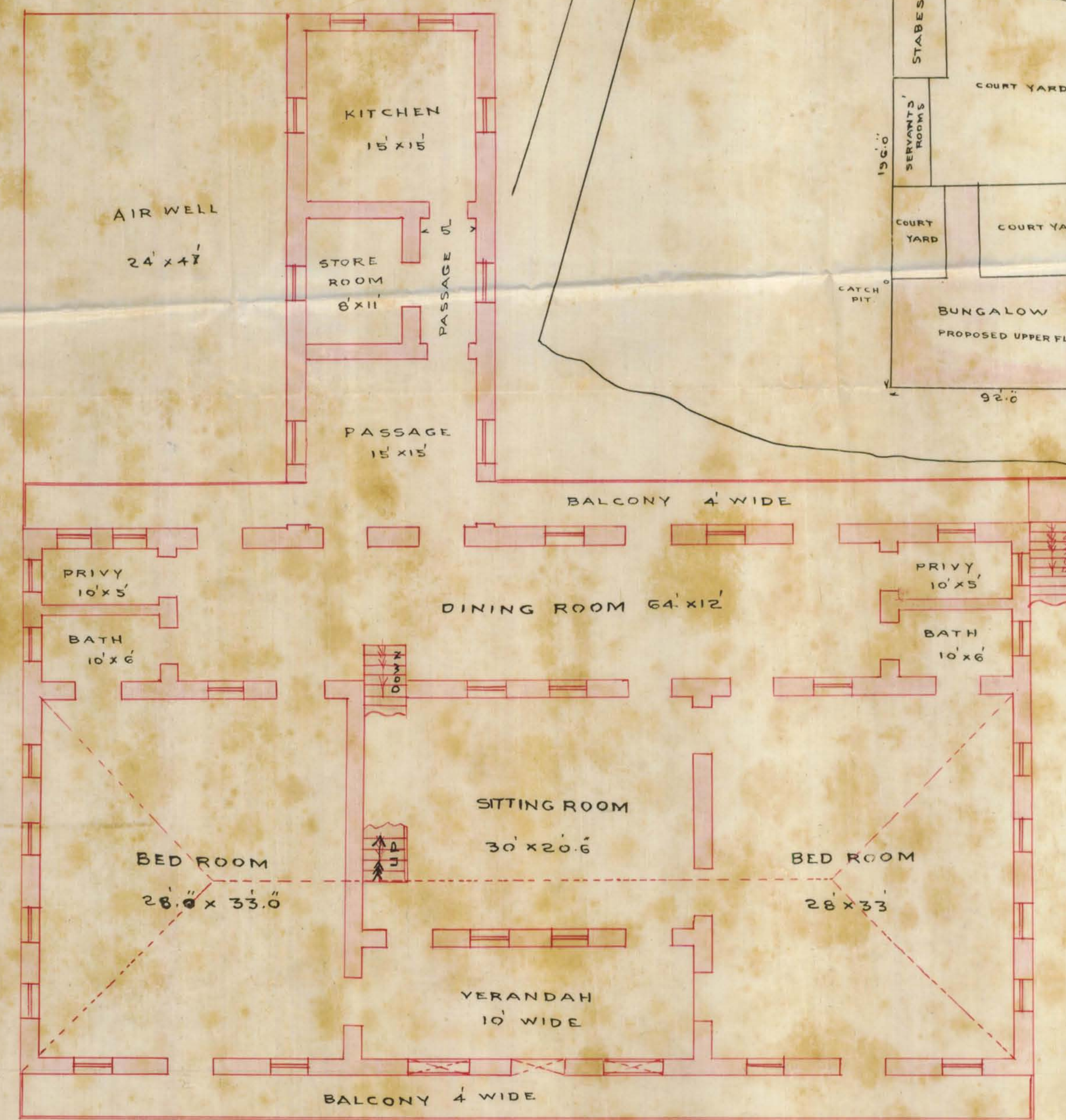
PLAN OF 1ST & 2ND FLOORS (PROPOSED)
