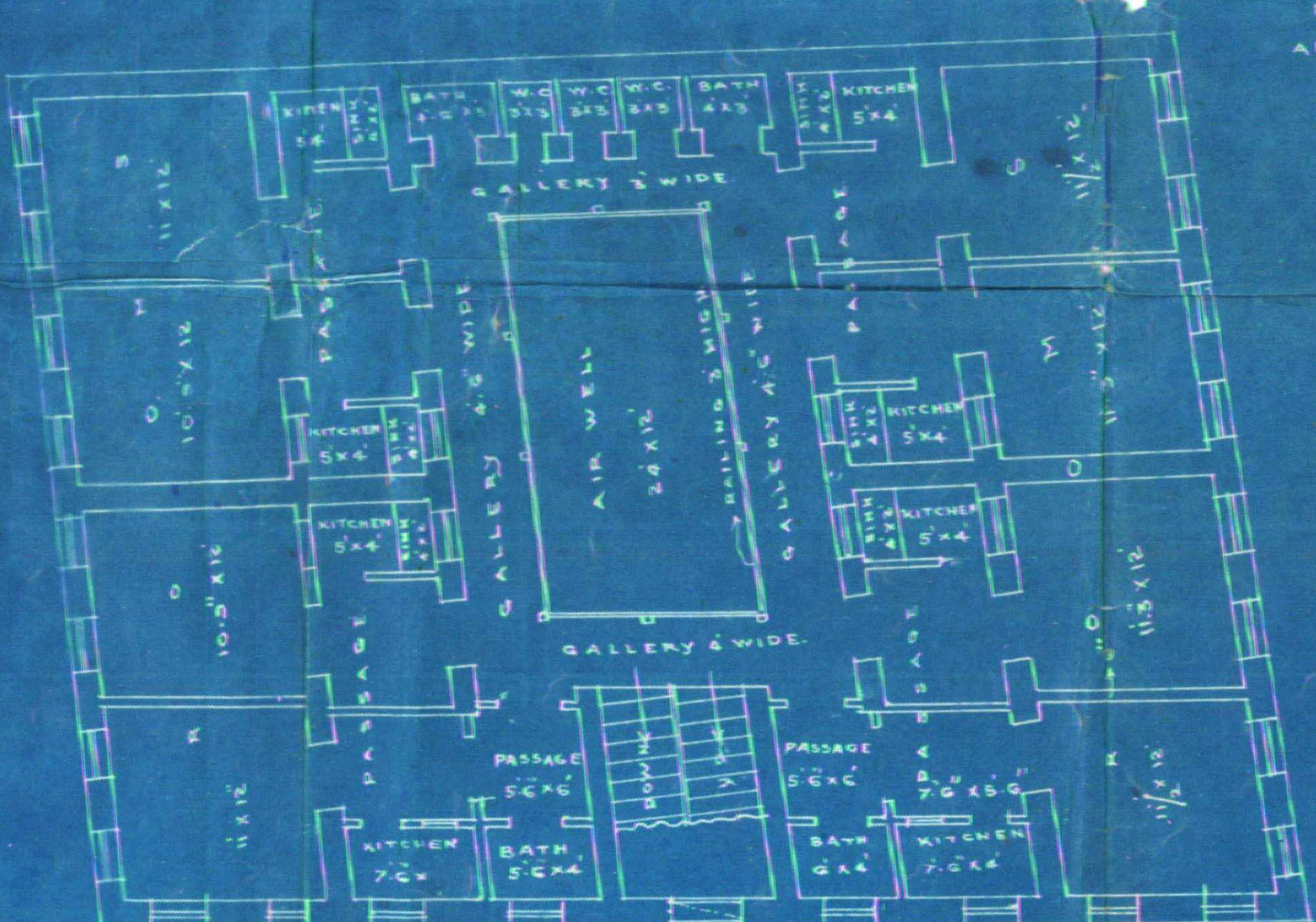
PLAN OF 1ST, 2ND & 3RD FLOORS.
