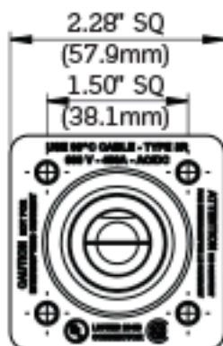
Typical Front for Male Panel Receptacle
