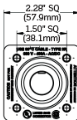
Typical Front for Female Panel Receptacle
