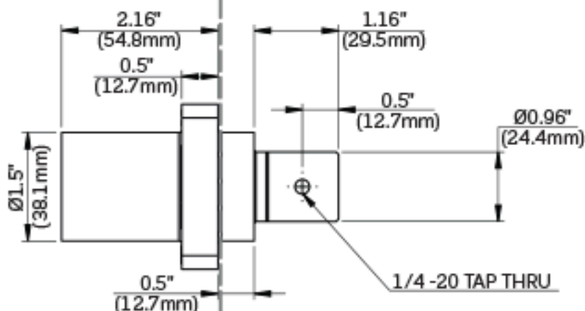
Typical for Bus Bar Termination (Top View)
