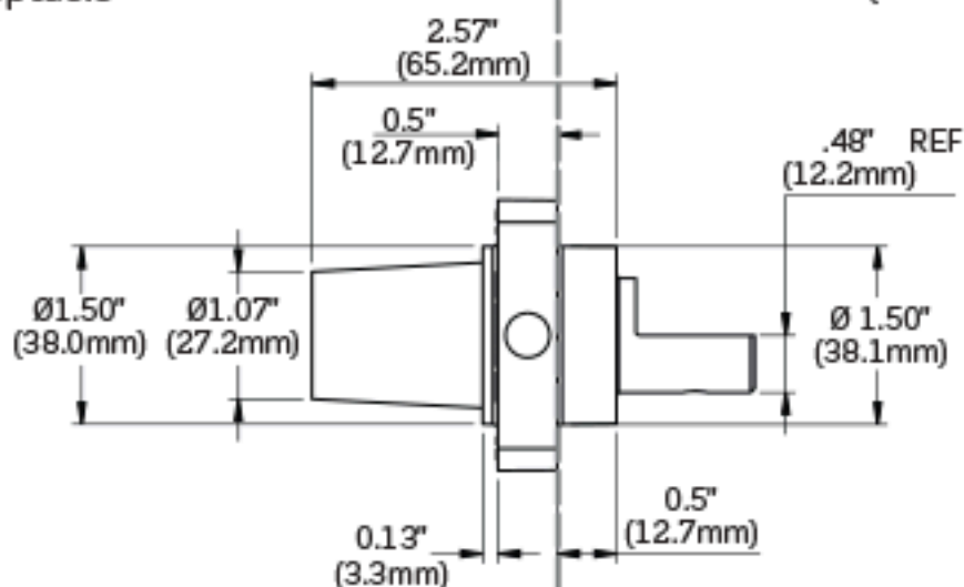
Typical for Bus Bar Termination (Side View)
