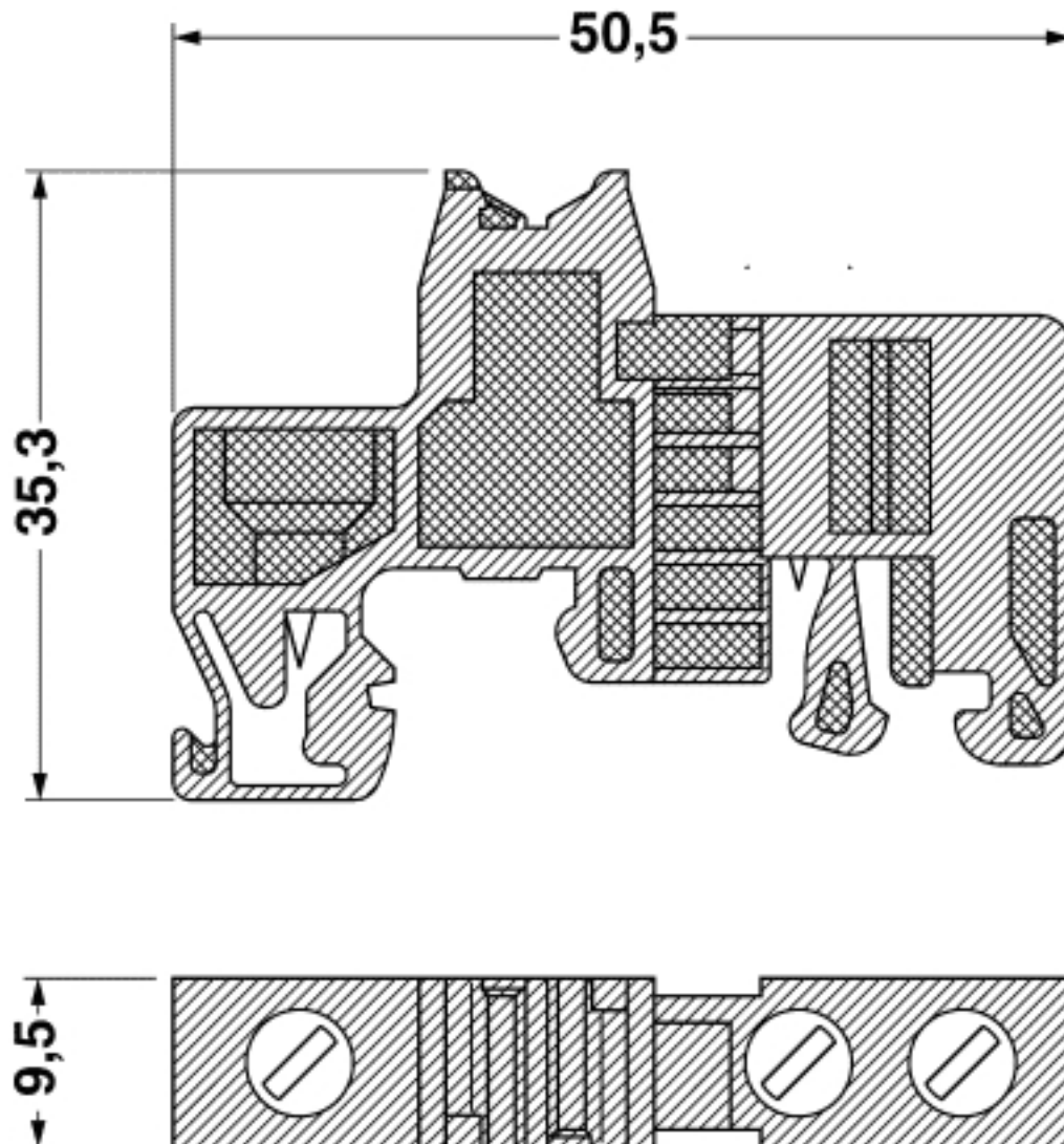
Dimensional drawing
