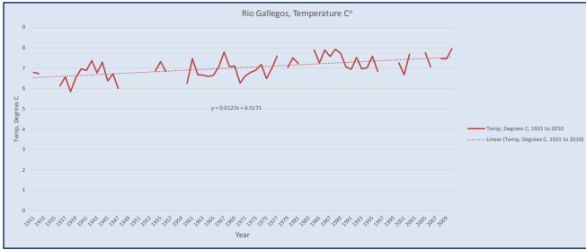
Figure 2. Southern Chile Weather Station Data
