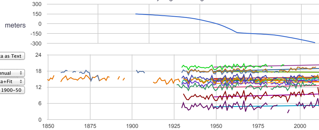
Erciyes glacier length
