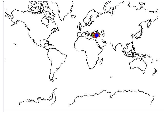
Erciyes glacier length
