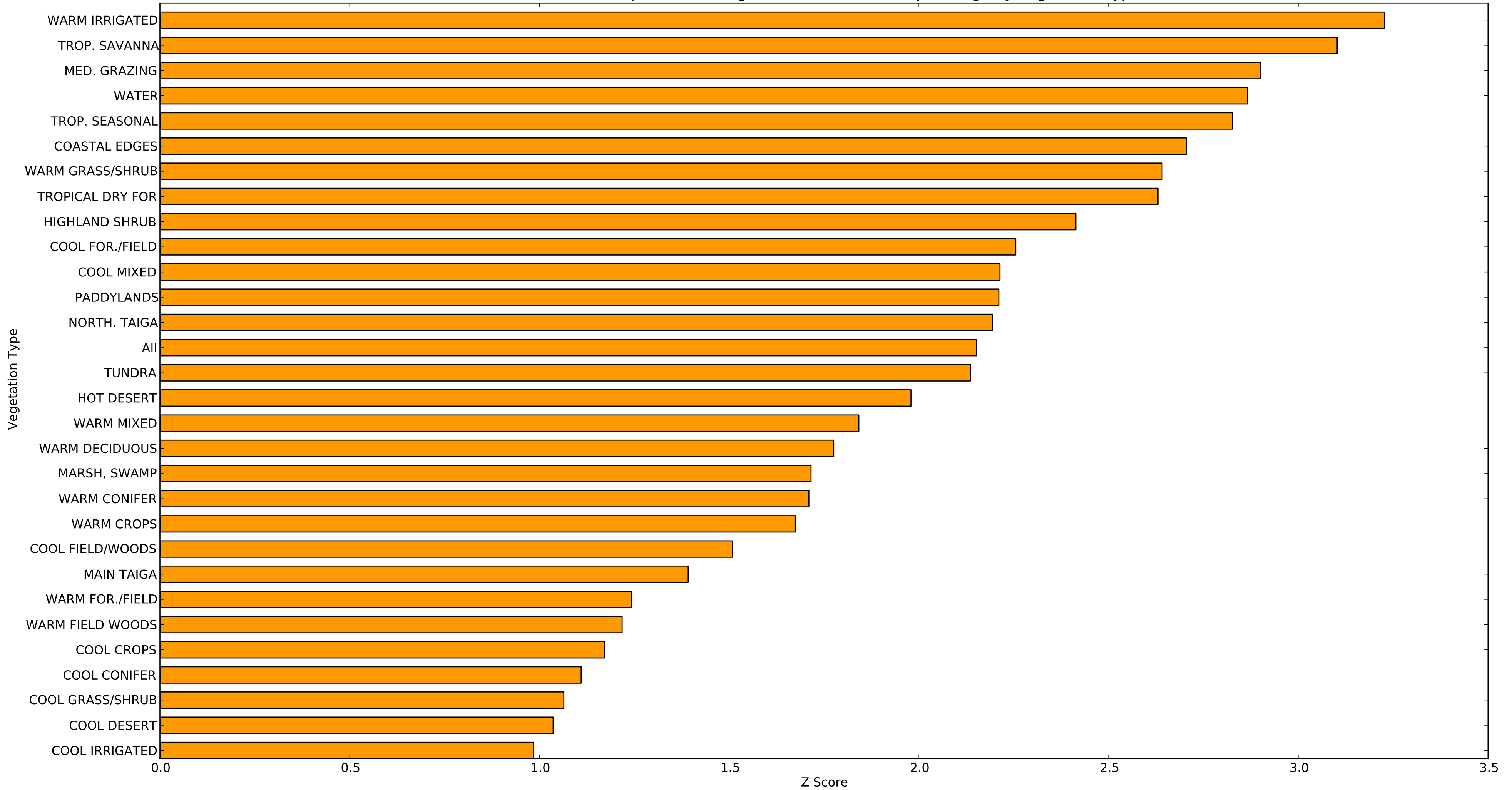
Z Score of Temperature Change (C) from 20th Century Average by Vegetation Type
