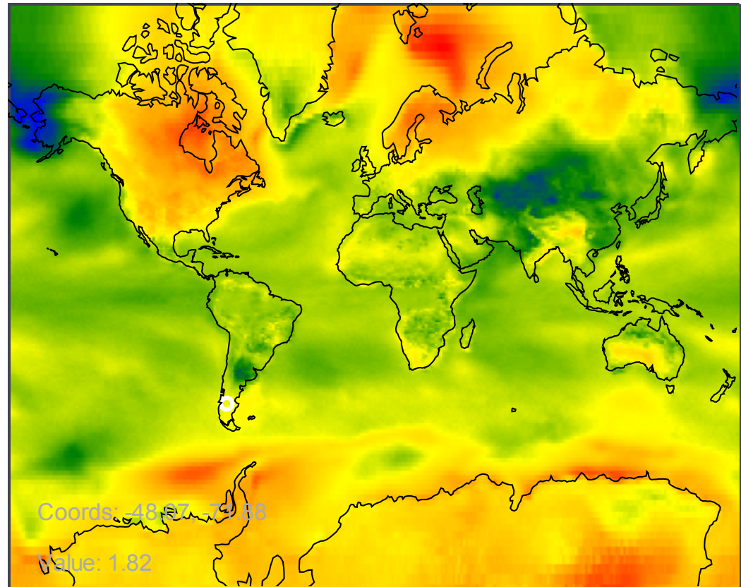
CCSM4 Surf Temp Annual Mean, 2012 Anomaly
