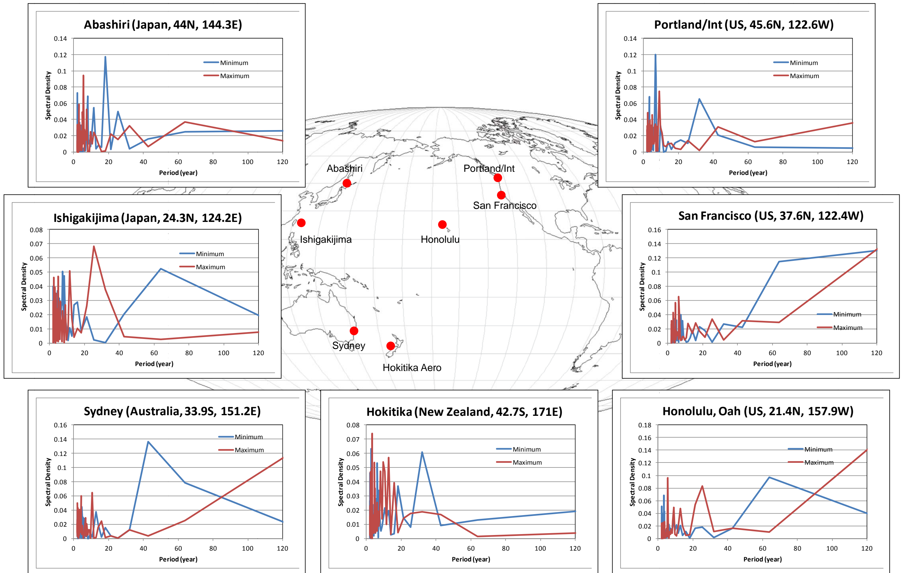
Figure 2 Power Spectra of Annual Temperature History
