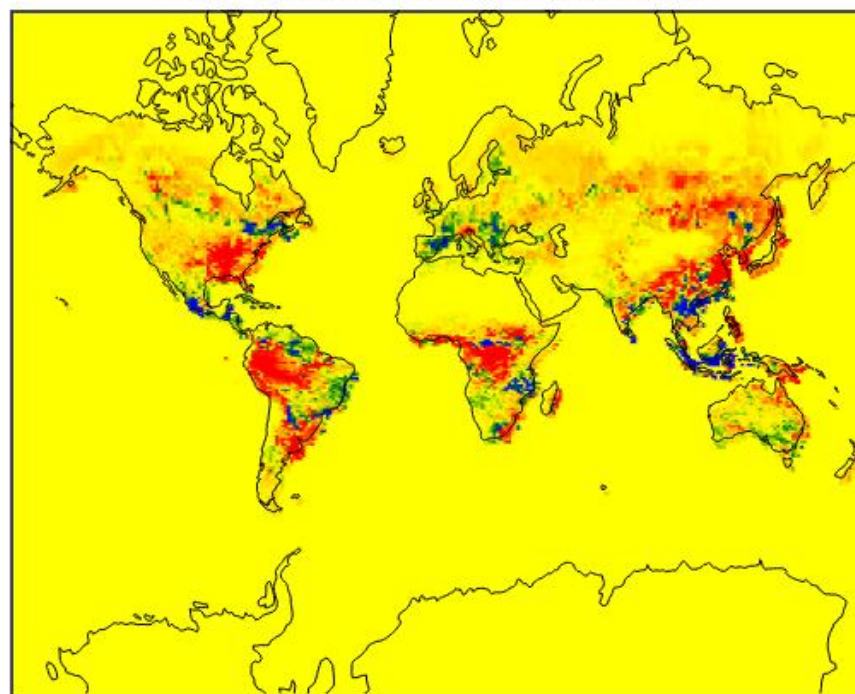
CCSM4 Leaf Index Annual Mean, 2099 Anomaly
