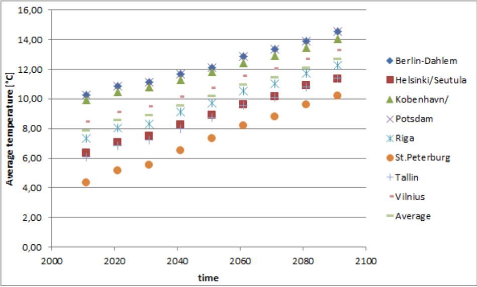
Graphic 1. Mean temperature decadal changes in the period of 2011-2100 according to five selected models.
