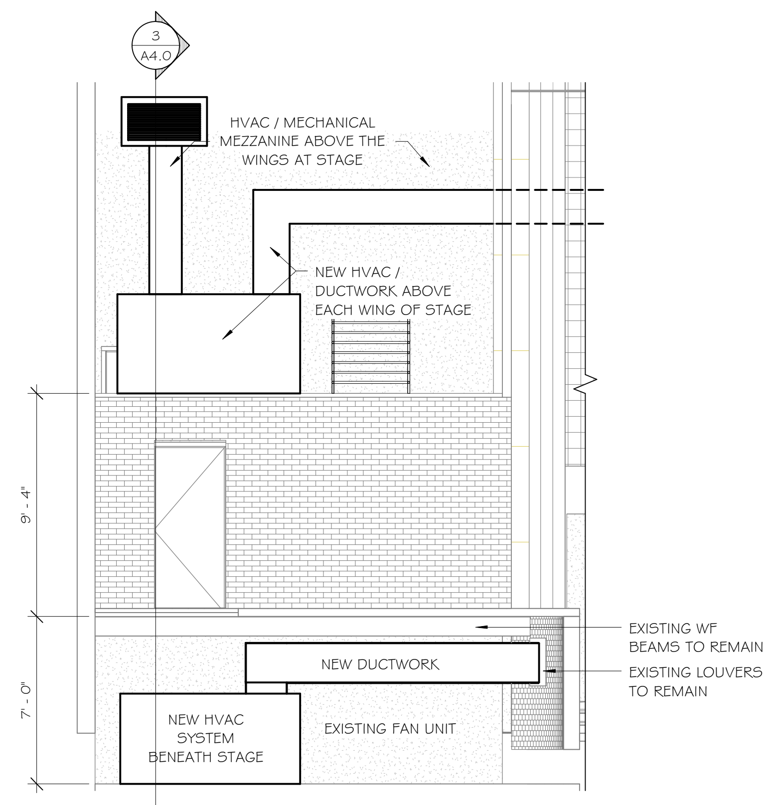
2 Section 2 1/4" = 1'-0"
