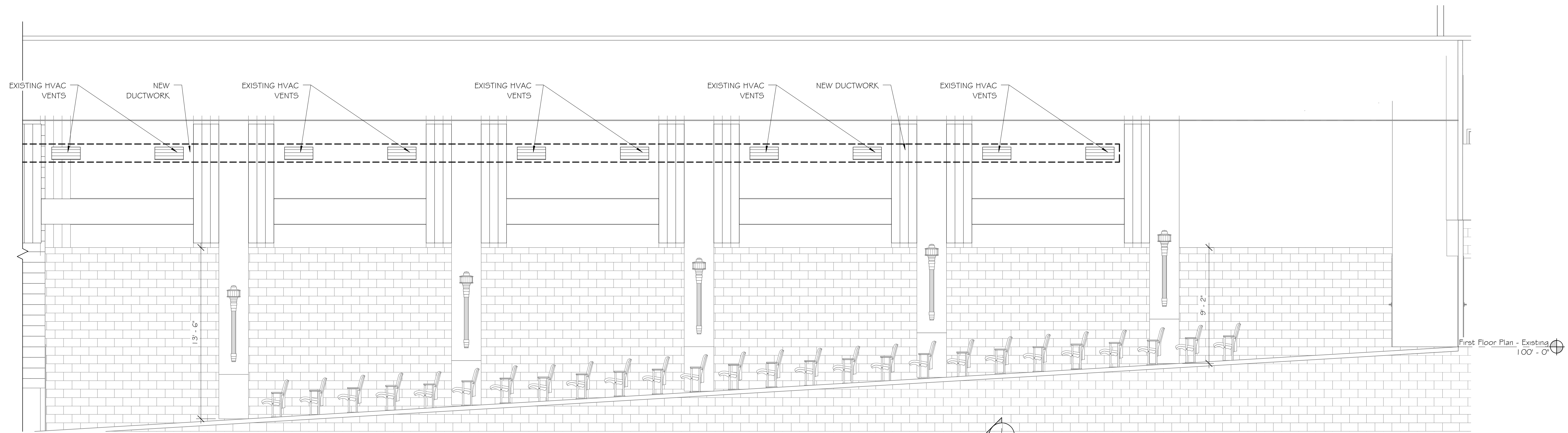
1 Section 1 1/4" = 1'-0"
