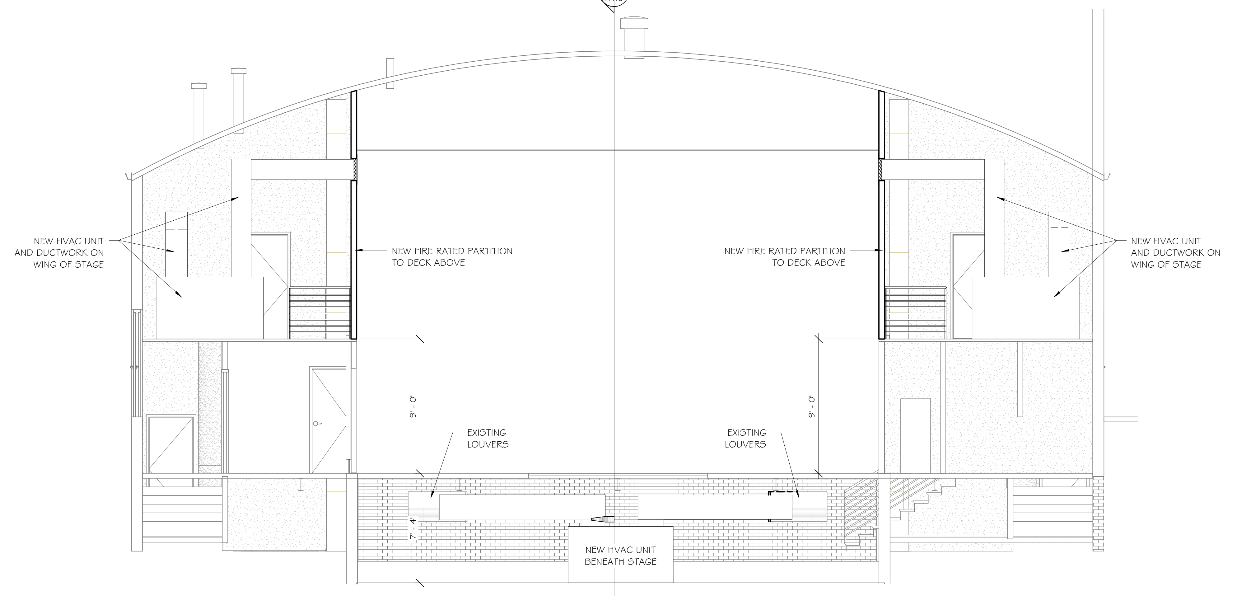
3 Section 3 1/4" = 1'-0"
