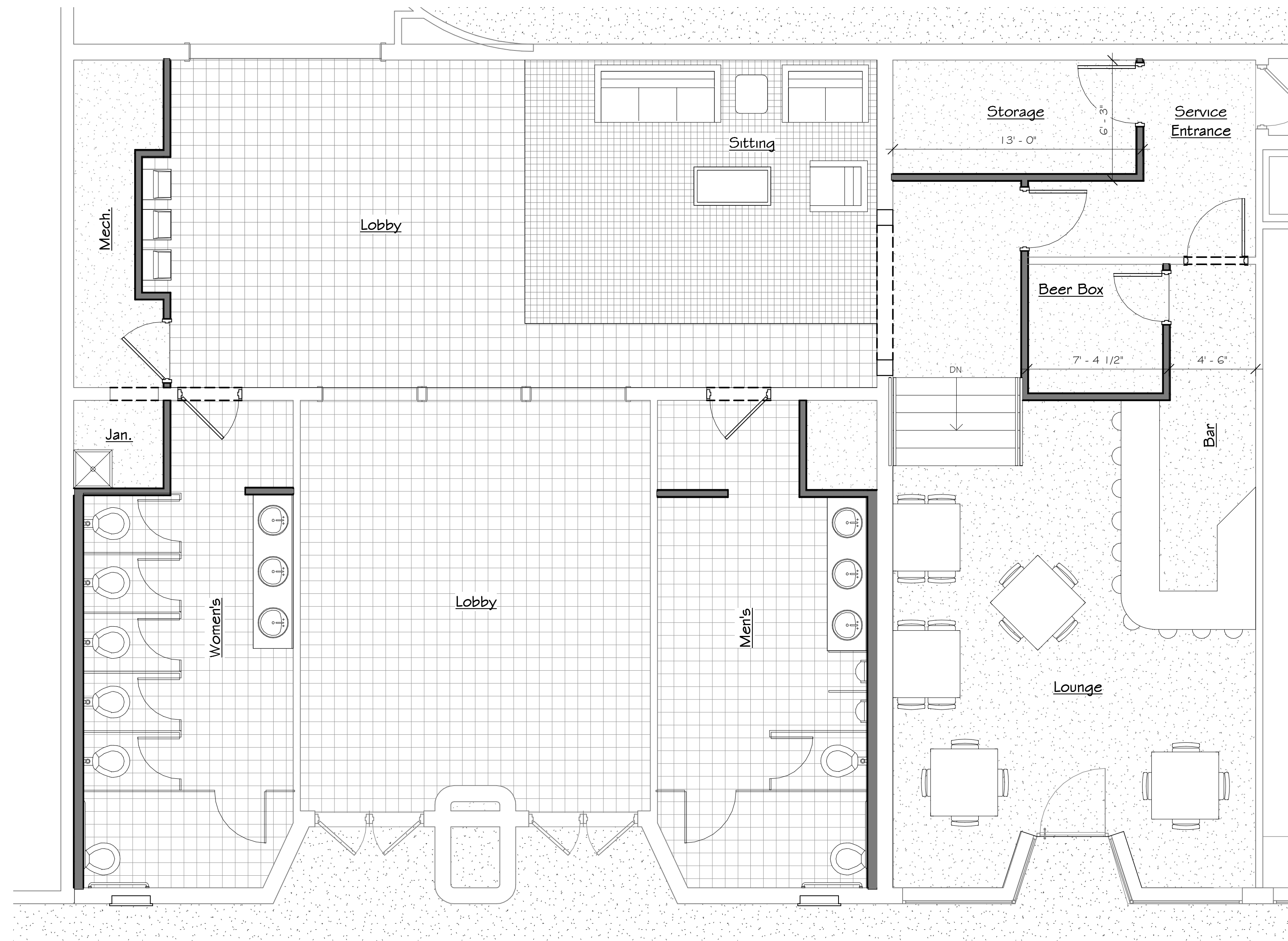
1 Lobby / Lounge Plan 1/4" = 1'-0"
