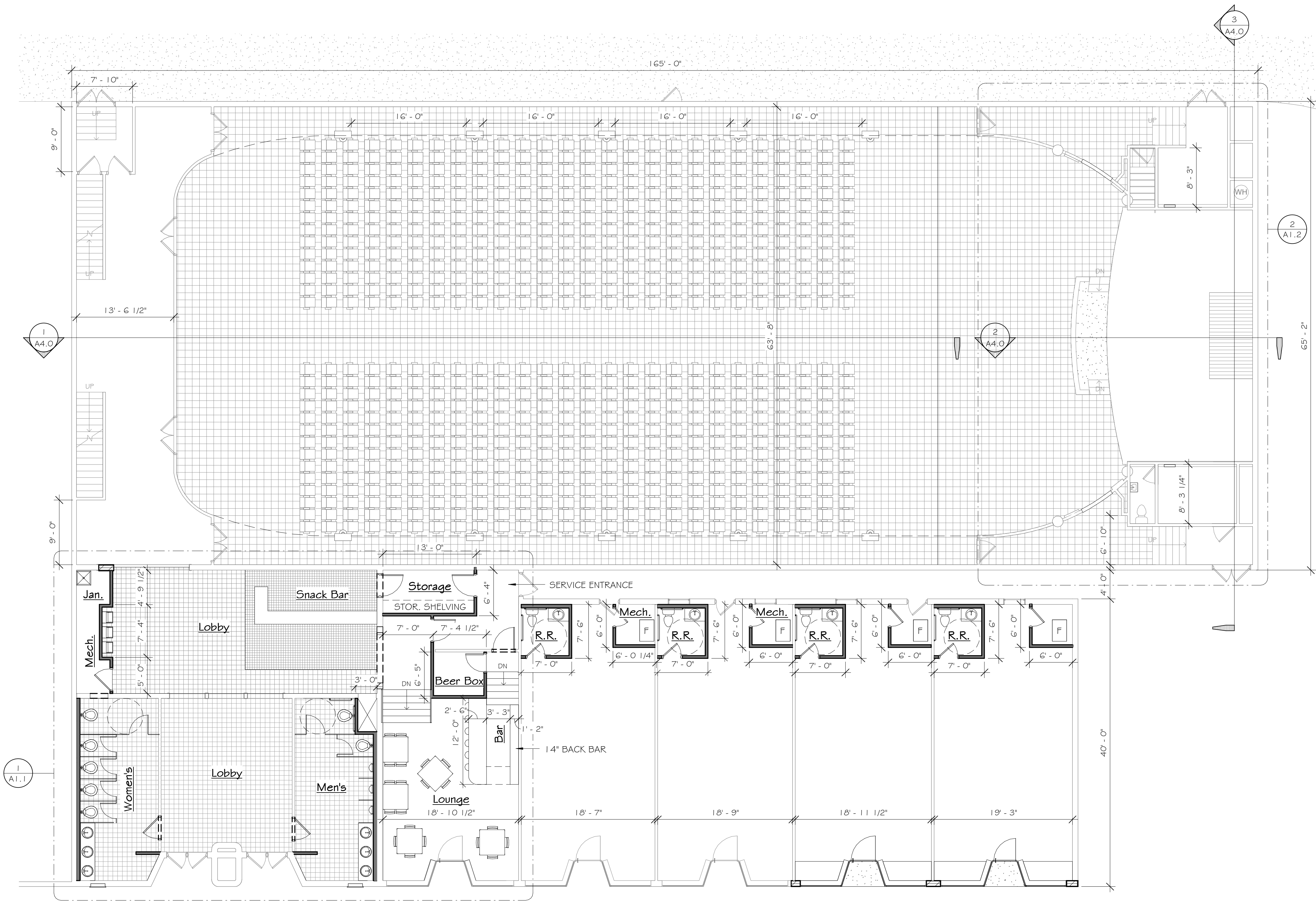
1 First Floor Plan - New Work 1/8" = 1'-0"
