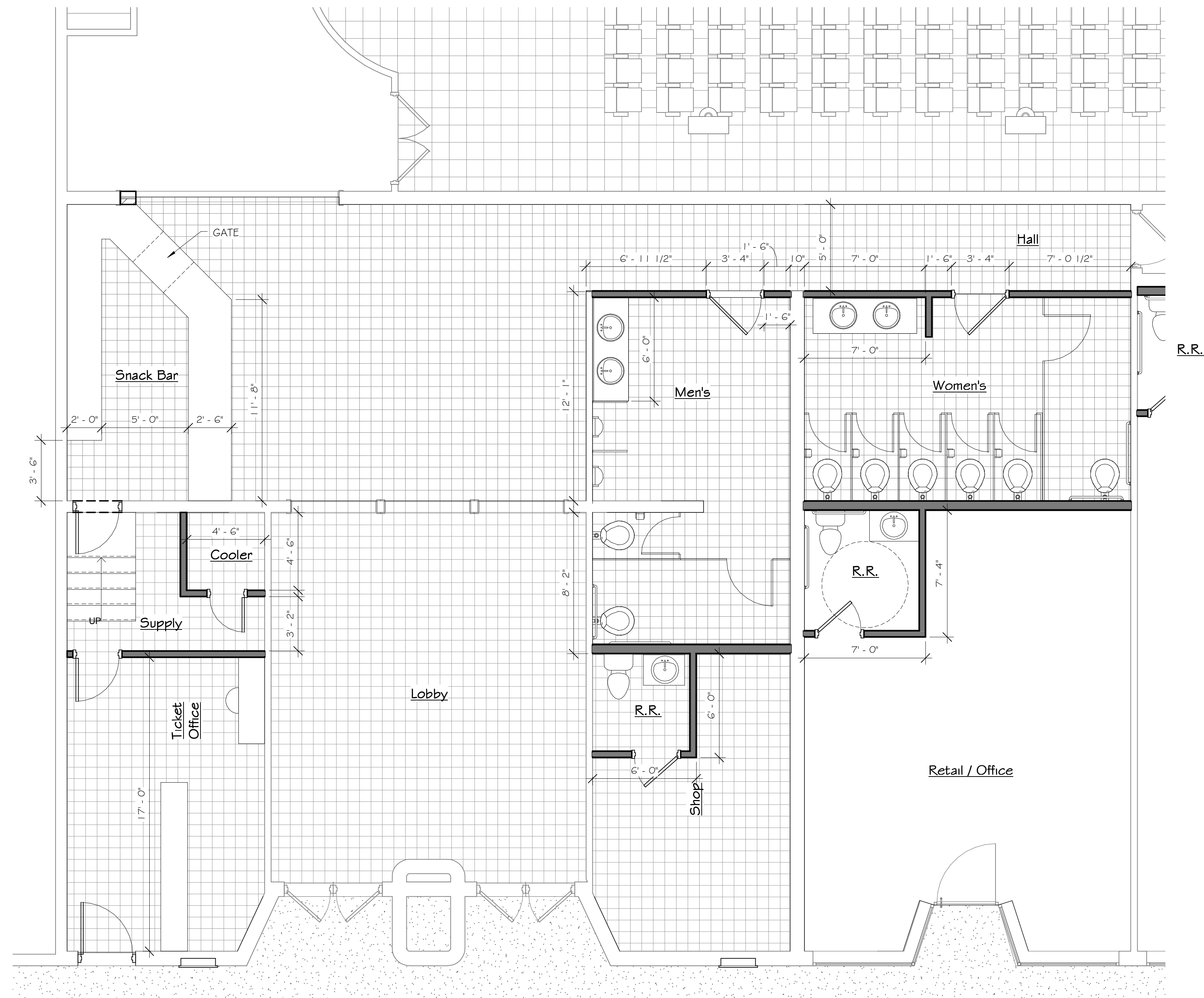
1 Lobby / Lounge Plan - New Work 1/4" = 1'-0"
