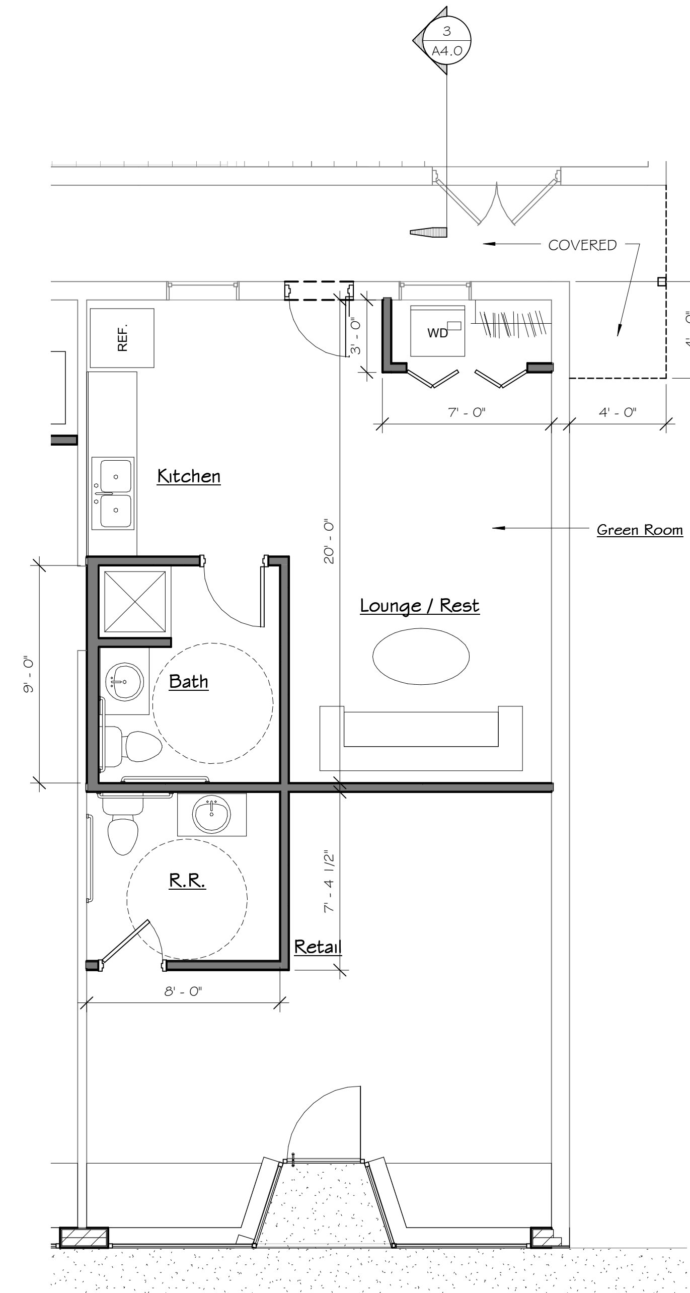
3 Green Room Plan - New Work 1/4" = 1'-0"
