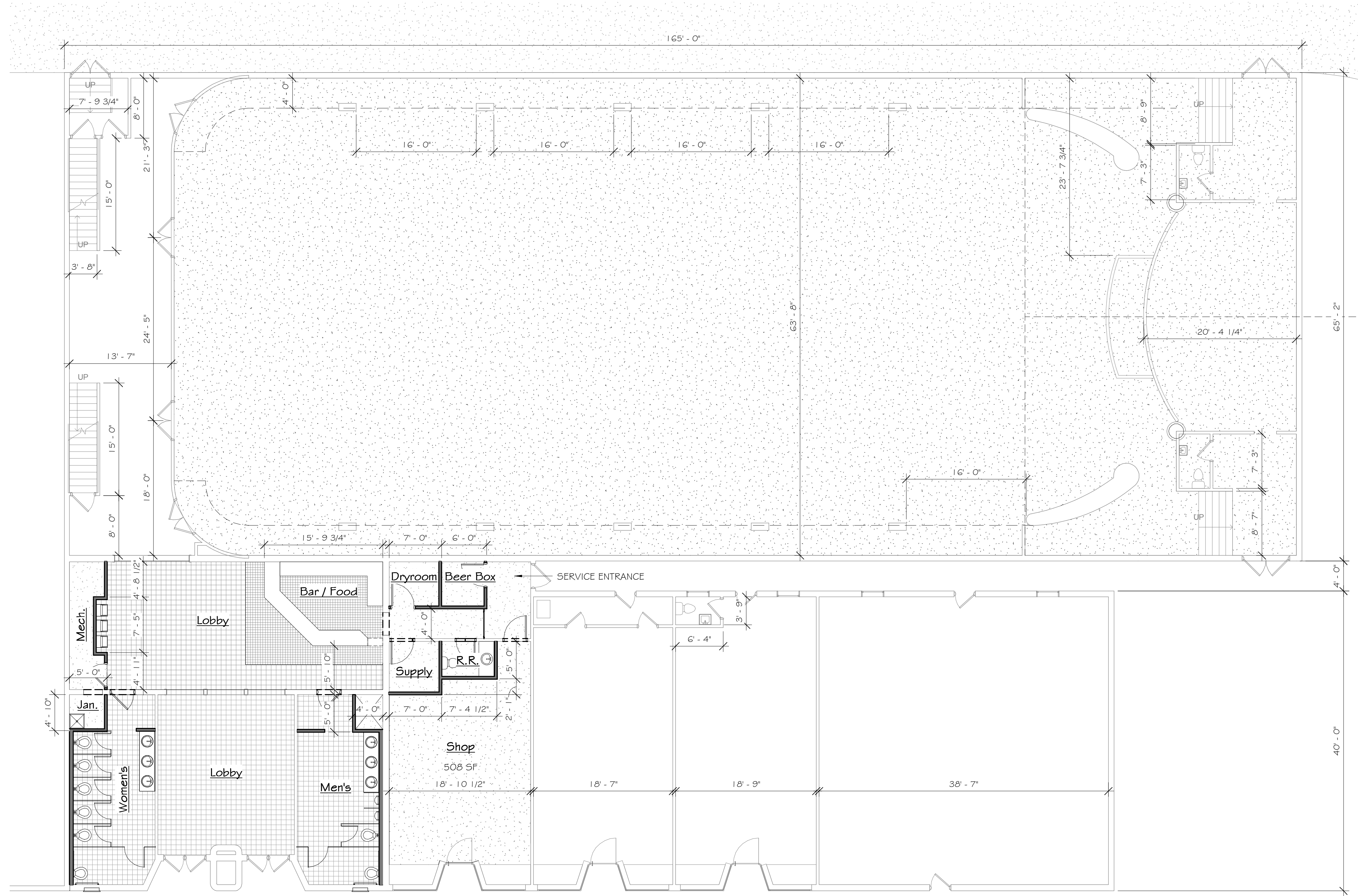
1 First Floor Plan - New Work 1/8" = 1'-0"
